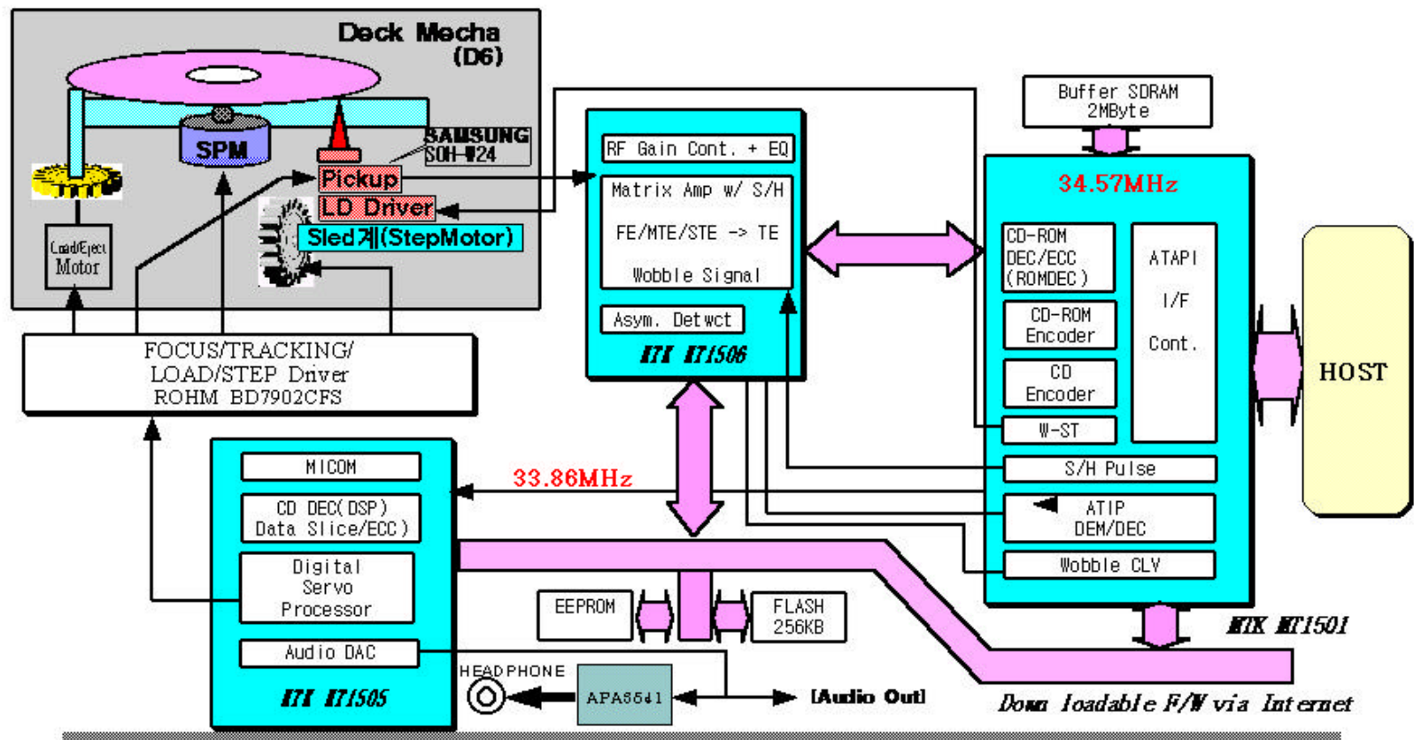
SW-224 Block Diagram
