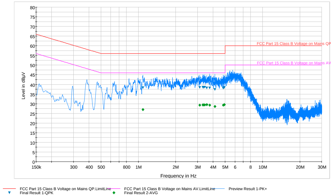
Plot 6-54. Line Conducted Plot with 802.11b (N)
