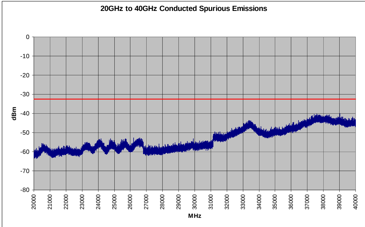
Plot 6-52. Conducted Spurious Plot (802.11a – Ch. 165)
