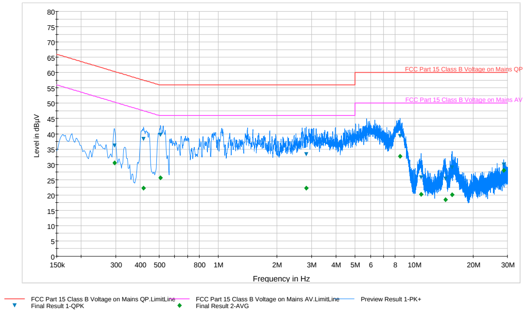
Plot 6-55. Line Conducted Plot with 802.11a (L1)
