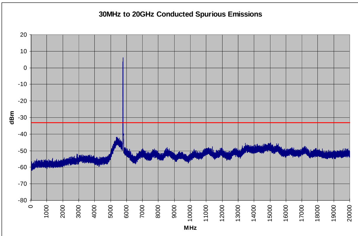
Plot 6-49. Conducted Spurious Plot (802.11a – Ch. 157)
