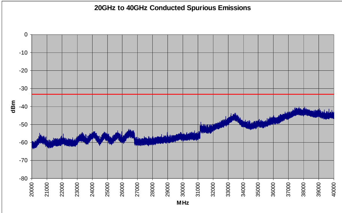
Plot 6-48. Conducted Spurious Plot (802.11a – Ch. 149)
