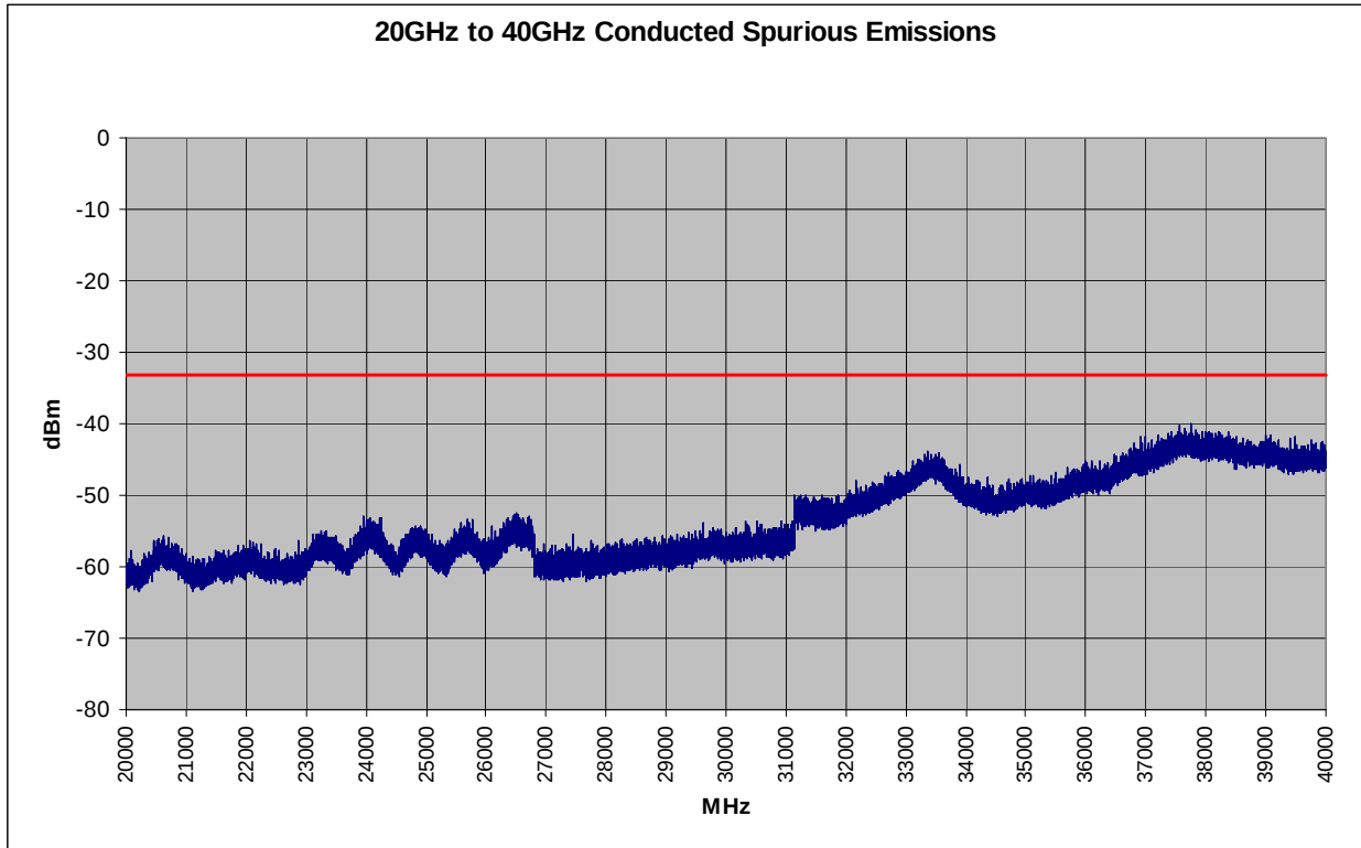
Plot 6-50. Conducted Spurious Plot (802.11a – Ch. 157)
