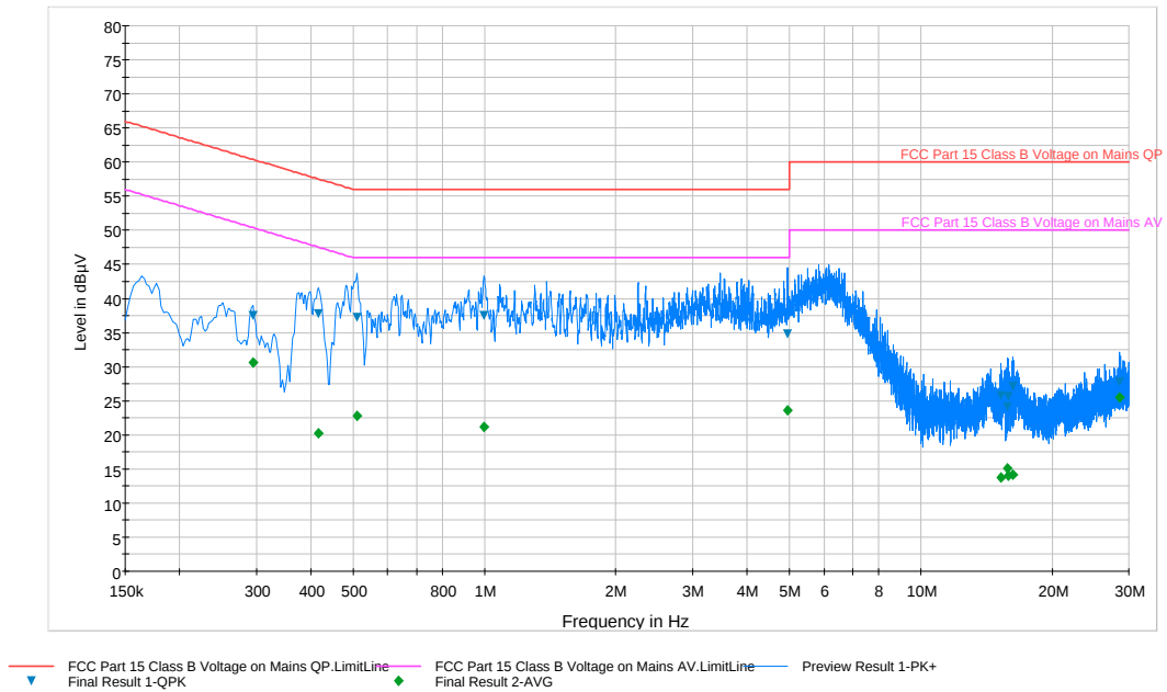
Plot 6-53. Line Conducted Plot with 802.11b (L1)
