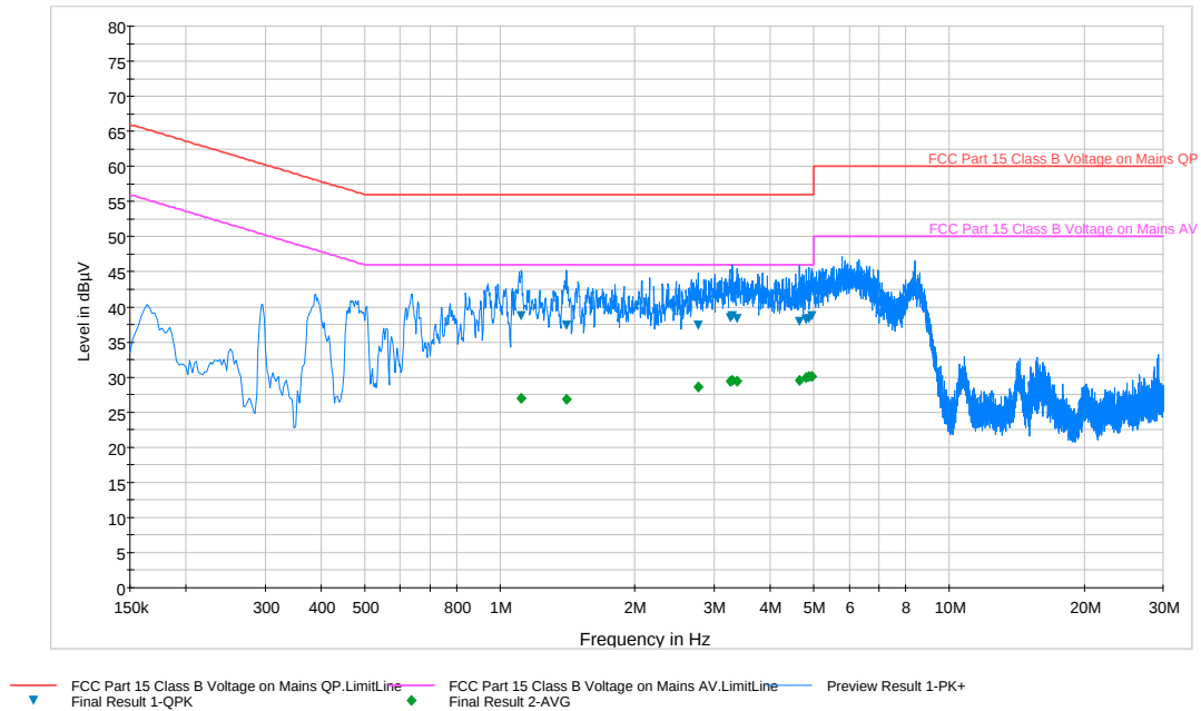
Plot 6-56. Line Conducted Plot with 802.11a (N)
