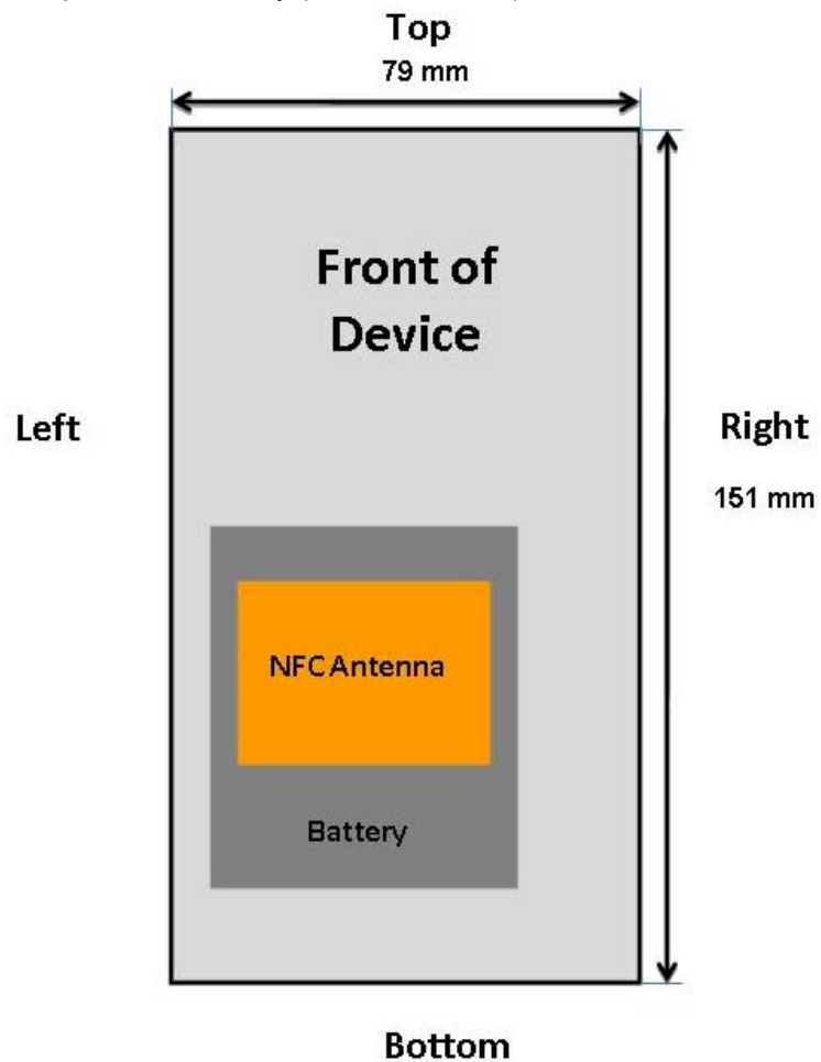
Figure 1-2 NFC Antenna Location
