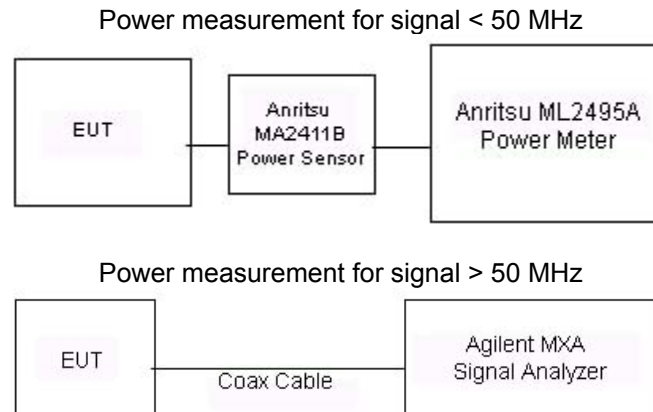
Figure 8-3 Power Measurement Setup
