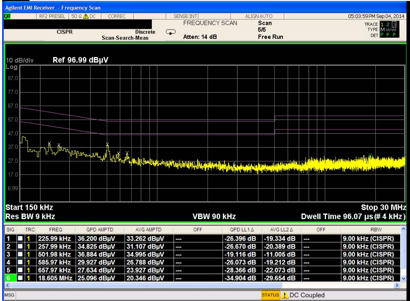
Plot 6-140. Line Conducted Plot with 802.11a (N)
