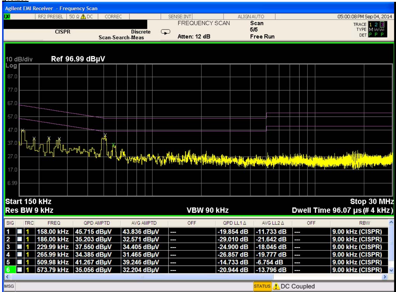
Plot 6-139. Line Conducted Plot with 802.11a (L1)
