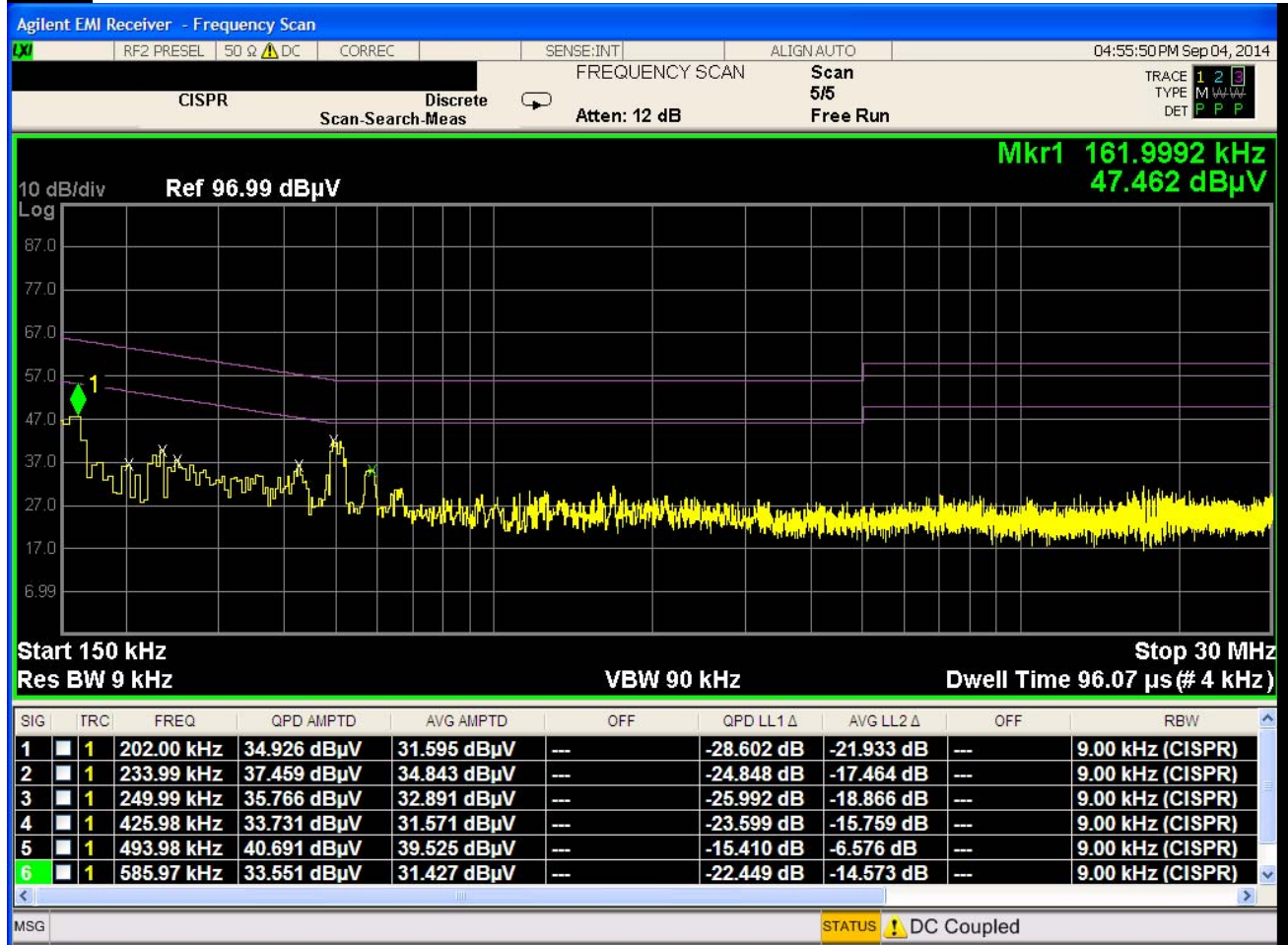
Plot 6-138. Line Conducted Plot with 802.11b (N)
