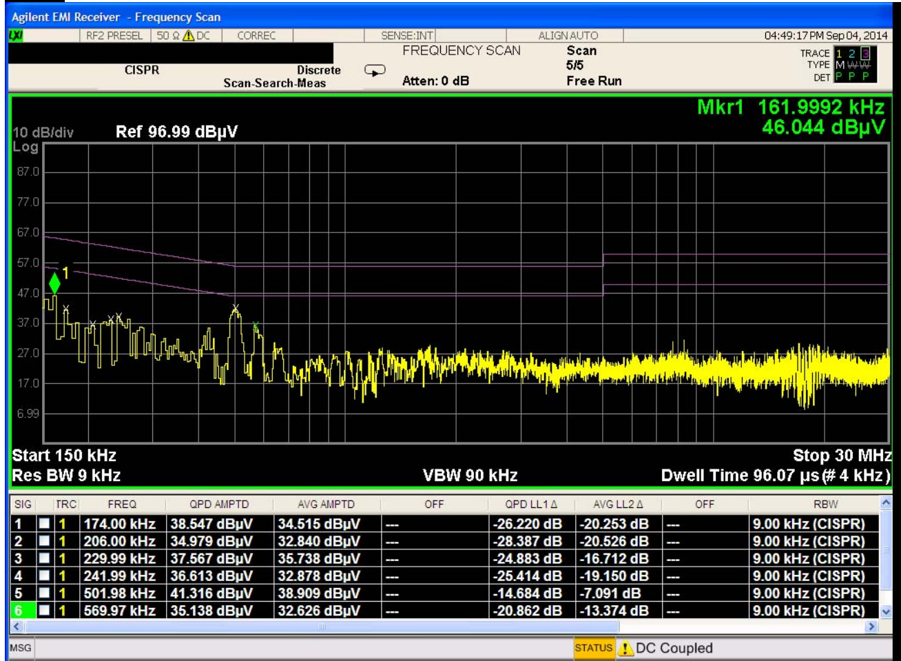
Plot 6-137. Line Conducted Plot with 802.11b (L1)
