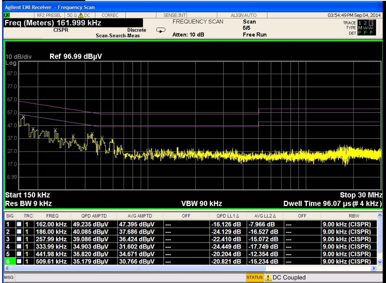
Plot 6-20. Line Conducted Plot with Bluetooth LE (L1)
