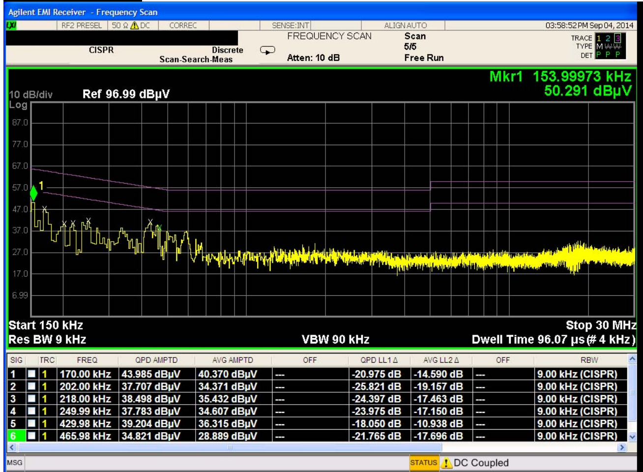
Plot 6-21. Line Conducted Plot with Bluetooth LE (N)
