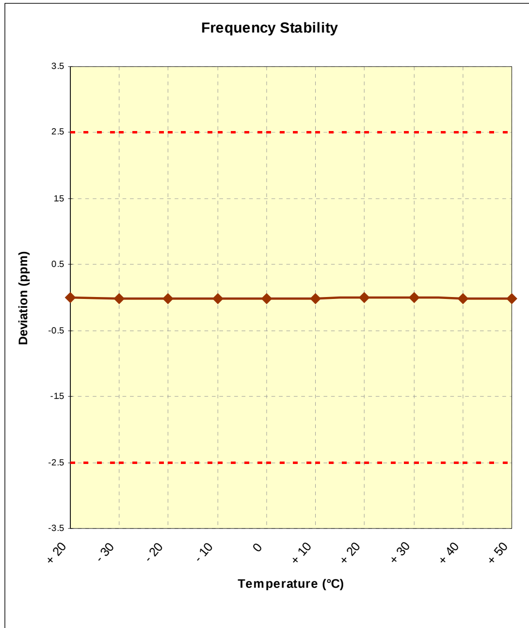
Figure 6-2. Frequency Stability Graph (PCS GSM Mode – Ch. 661)
