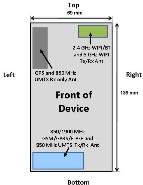
Figure 1-1 DUT Antenna Locations
