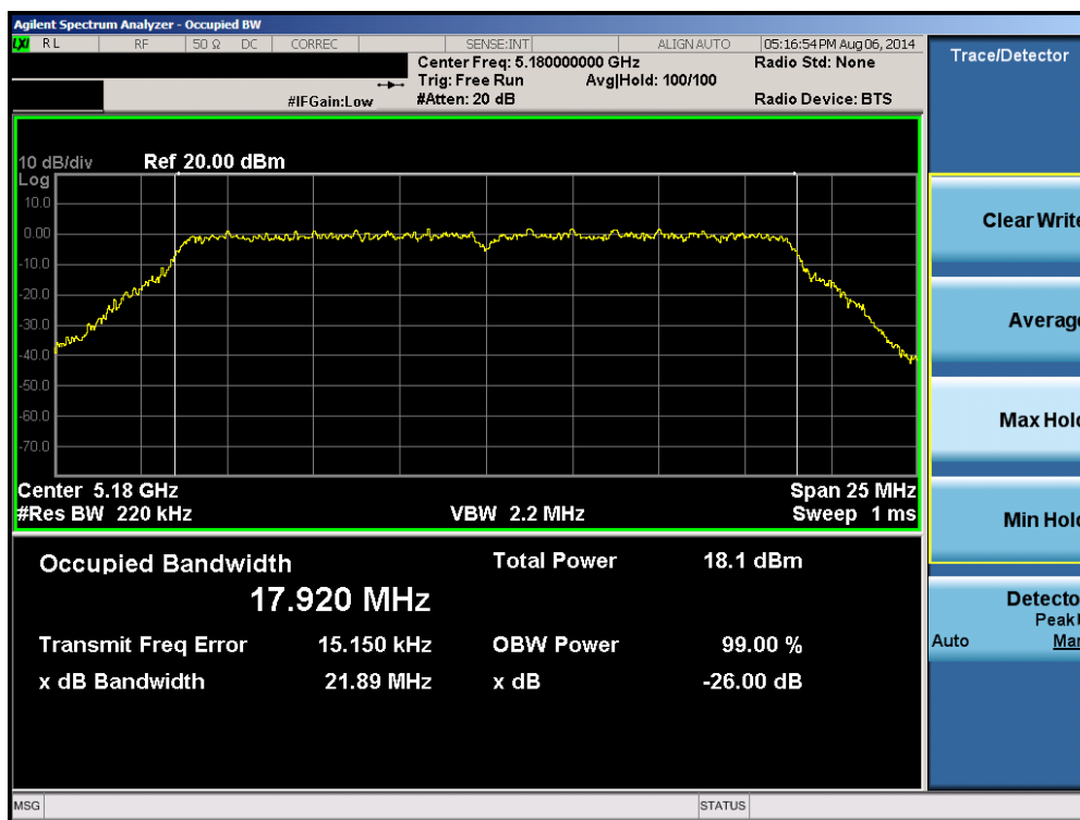
Plot 6-38. 26dB Bandwidth Plot (20MHz BW 802.11n (UNII Band 1) – Ch. 36)
