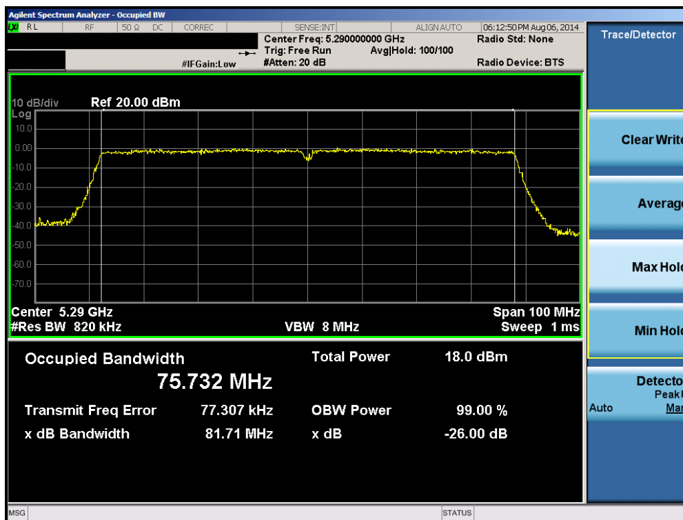
Plot 6-52. 26dB Bandwidth Plot (80MHz BW 802.11ac (UNII Band 2A) – Ch. 58)
