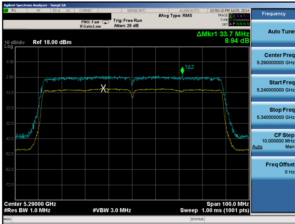
Plot 6-126. Peak Excursion Ratio Plot (80MHz BW 802.11ac (UNII Band 2A) – Ch. 58)
