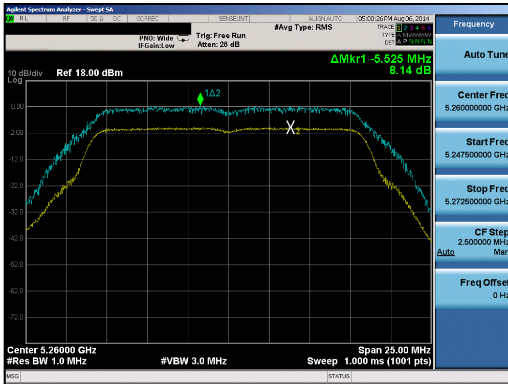
Plot 6-131. Peak Excursion Ratio Plot (802.11a (UNII Band 2A) – Ch. 52)
