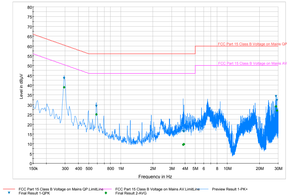
Plot 6-69. Line Conducted Plot with 802.11a (L1)
