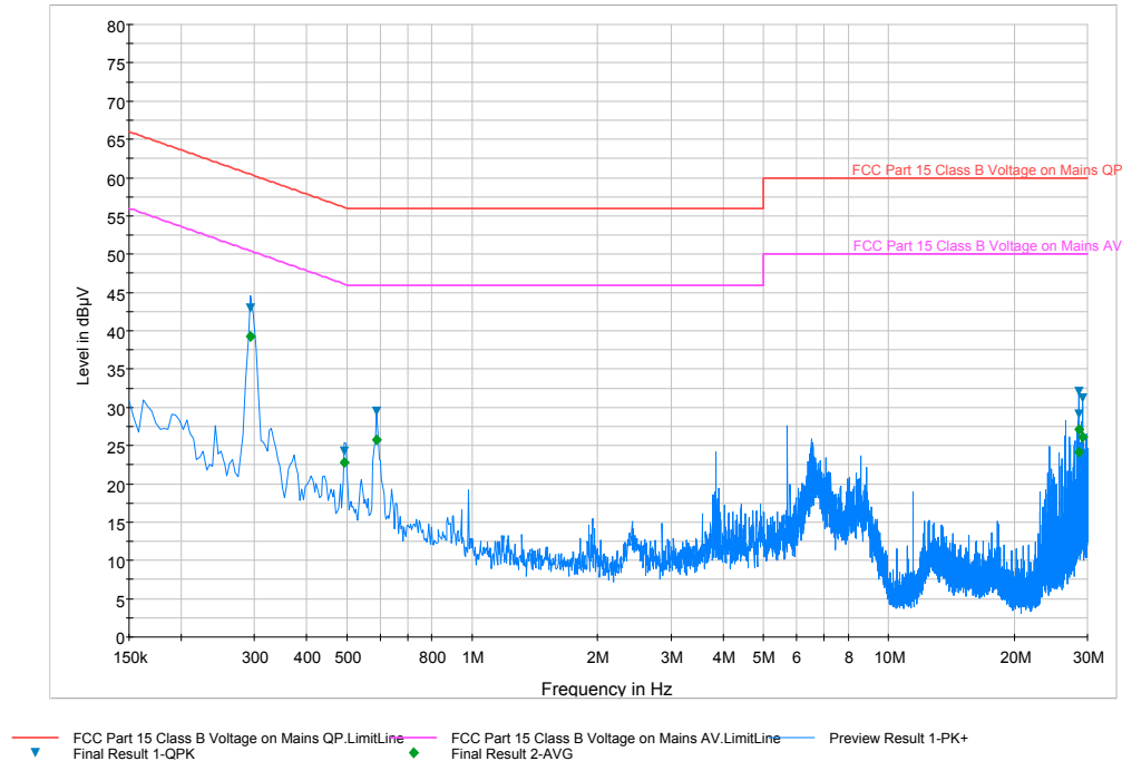
Plot 6-70. Line Conducted Plot with 802.11a (N)
