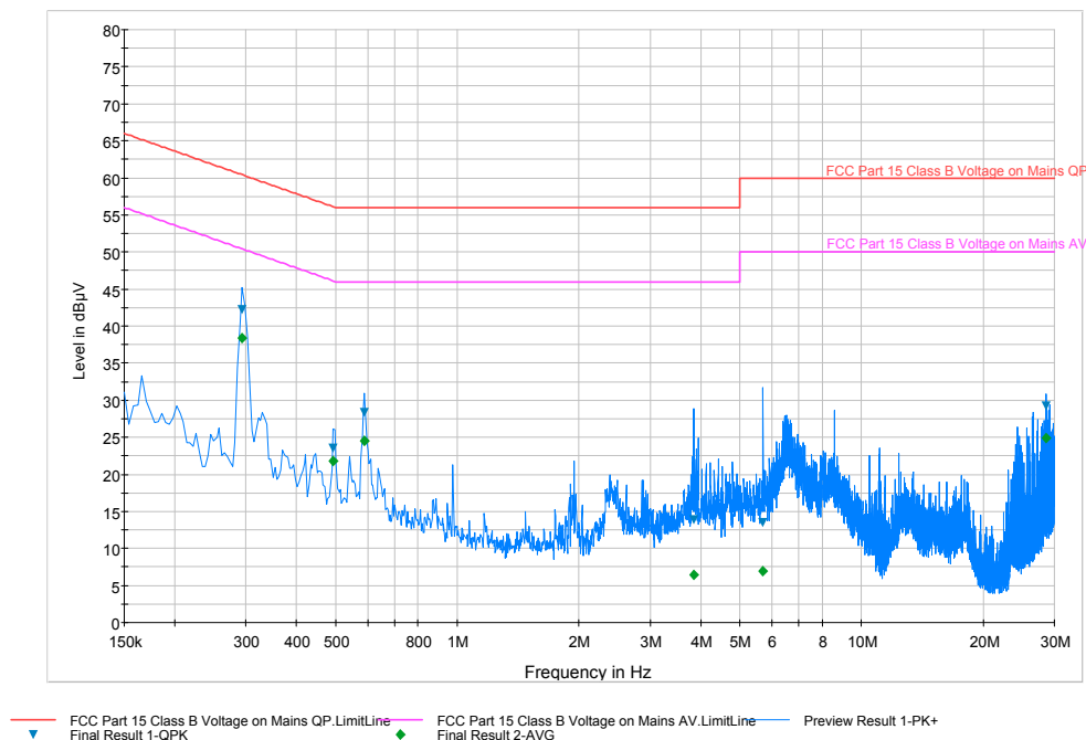
Plot 6-68. Line Conducted Plot with 802.11b (N)
