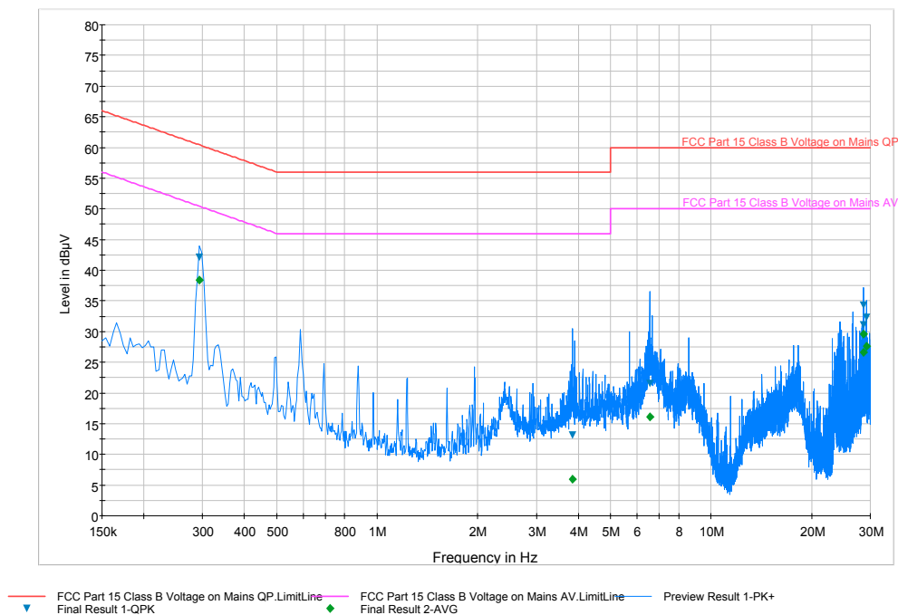
Plot 6-67. Line Conducted Plot with 802.11b (L1)
