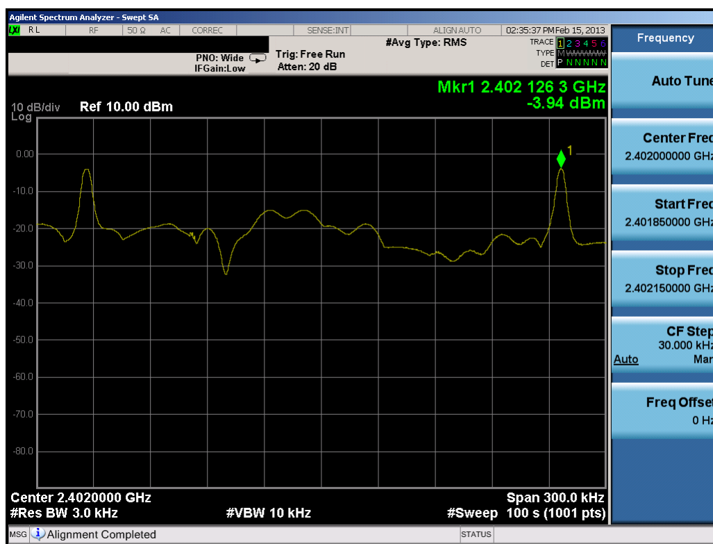
Plot 6-4. Power Spectral Density Plot (Bluetooth (LE) – Ch. 0)
