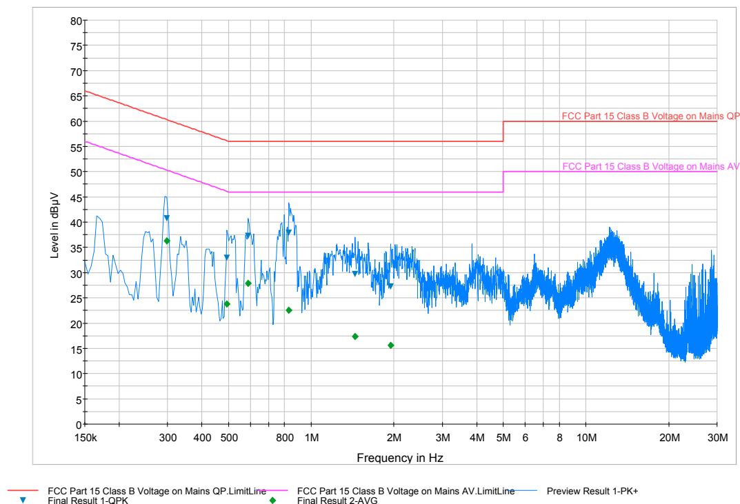
Plot 6-19. Line Conducted Plot with Bluetooth LE (L1)
