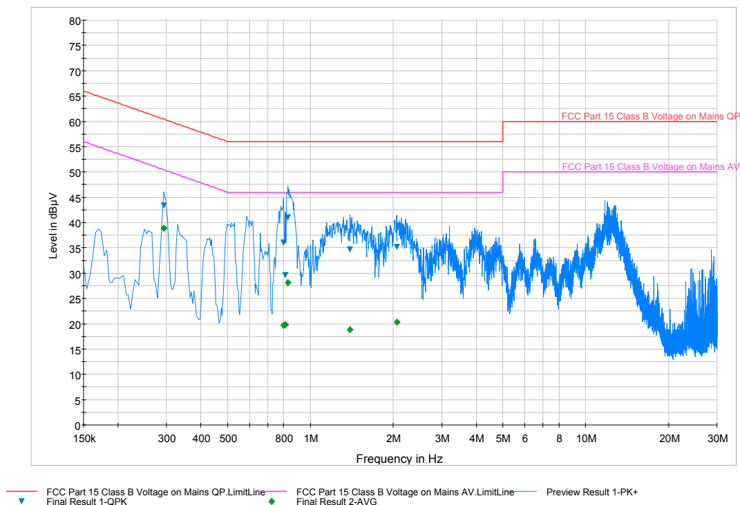
Plot 6-20. Line Conducted Plot with Bluetooth LE (N)
