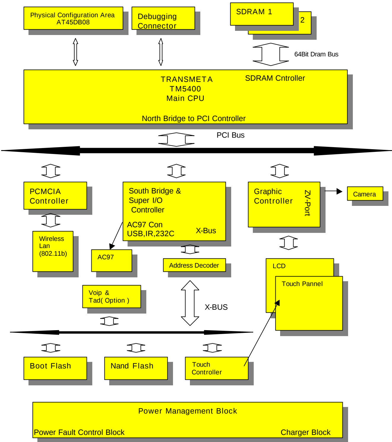
[ HomePad Block Diagram ]
