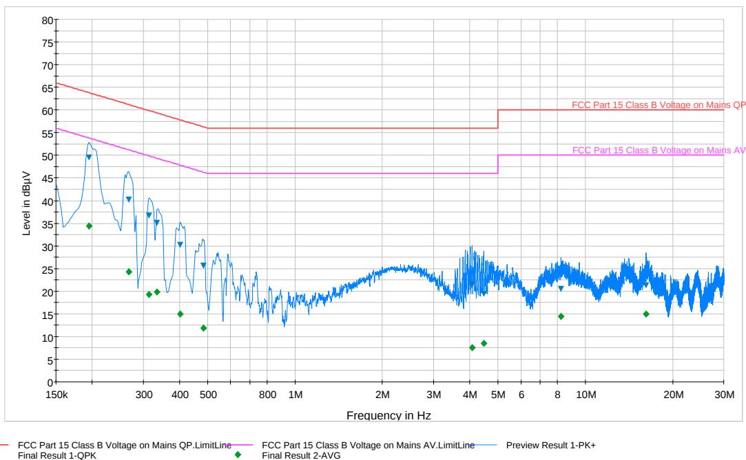
Plot 7-1. Line Conducted Test Plot (L1)
