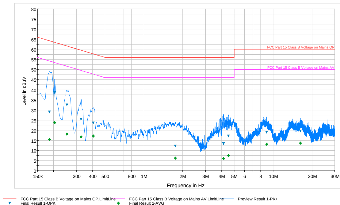
Plot 7-2. Line Conducted Test Plot (LN)
