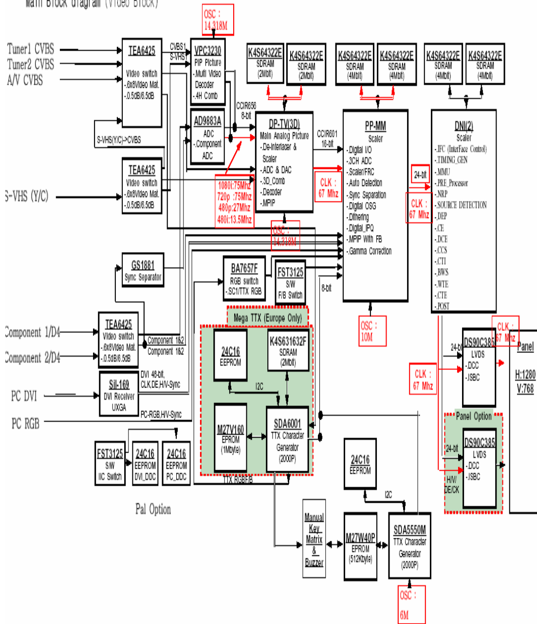
Main Block diagram (Video Block)
