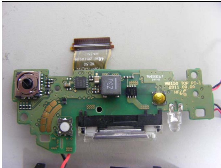
Top view of Flesh PCB
