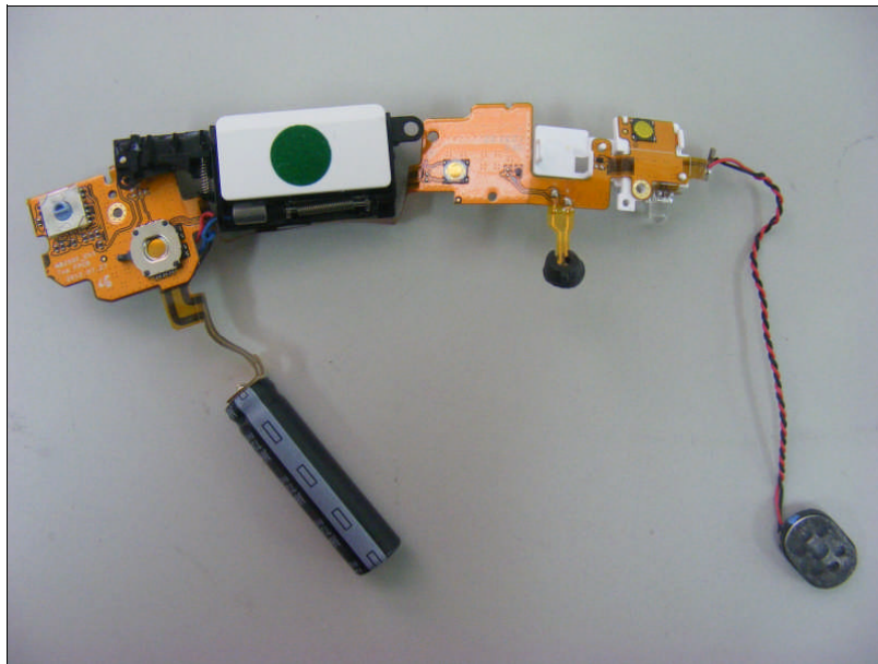
Top view of Sub FPCB
