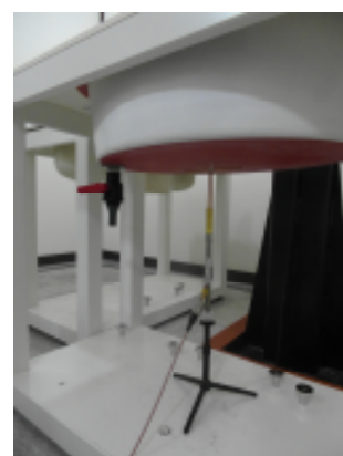
Fig c. Photo of the dipole Antenna
