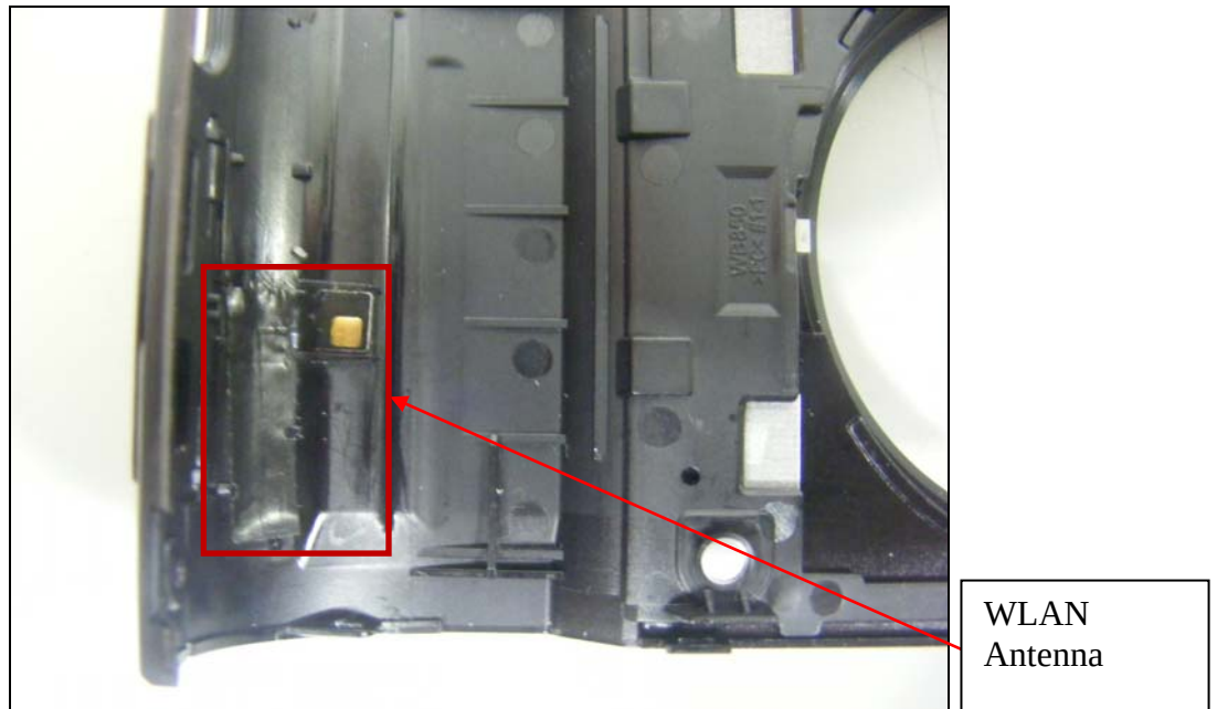
Bottom view of Antenna
