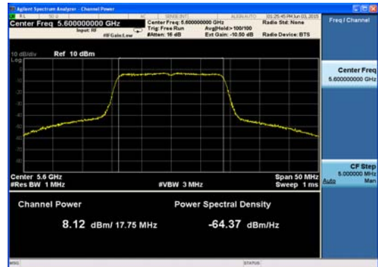
Ant : A1_802.11ac_VHT20 (1)
