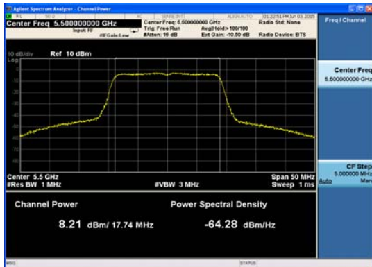
Ant : A1_802.11ac_VHT20 (1)
