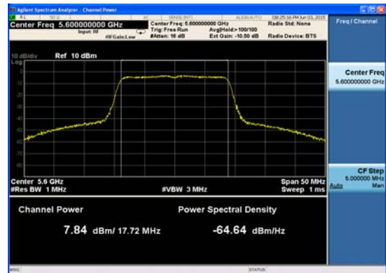
Ant : A3_802.11ac_VHT20 (1)
