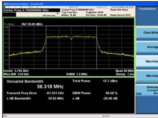
Ant : A3_802.11ac_VHT40 (2)
