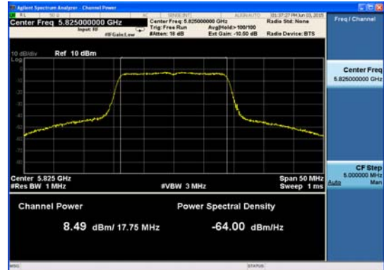
Ant : A1_802.11ac_VHT20 (2)
