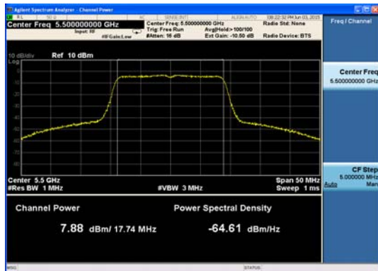
Ant : A3_802.11ac_VHT20 (1)
