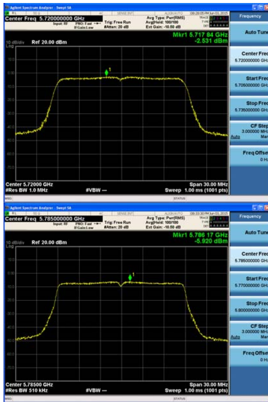
Ant : A3_802.11ac_VHT20 (2)
