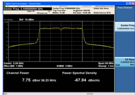
Ant : A3_802.11ac_HT40 (1)
