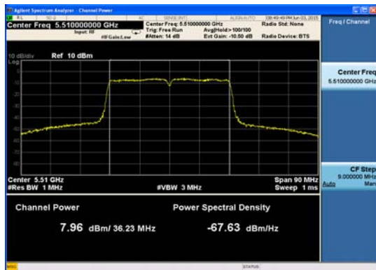
Ant : A3_802.11ac_HT40 (1)
