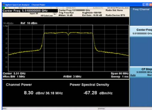
Ant : A2_802.11ac_HT40 (1)
