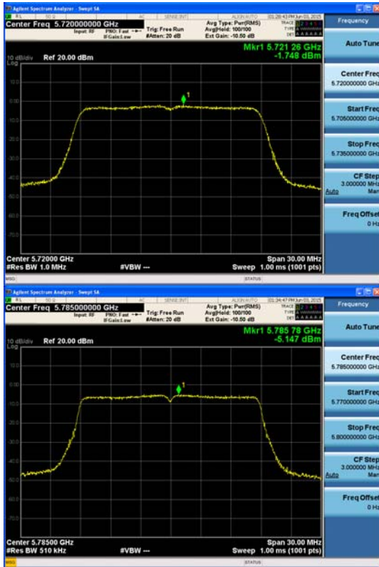
Ant : A1_802.11ac_VHT20 (2)
