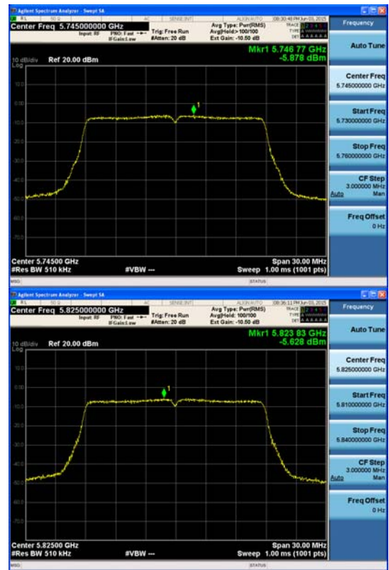
Ant : A3_802.11ac_VHT20 (2)
