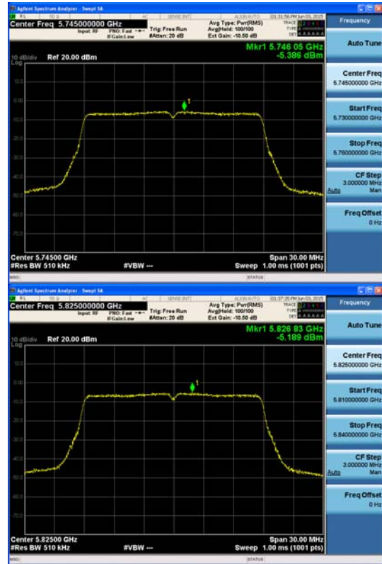
Ant : A1_802.11ac_VHT20 (2)
