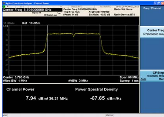
Ant : A3_802.11ac_HT40 (2)
