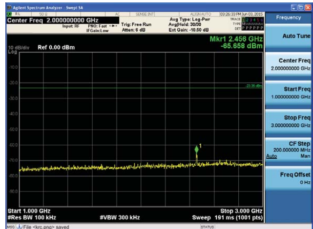
5745MHz 1GHz~3GHz
