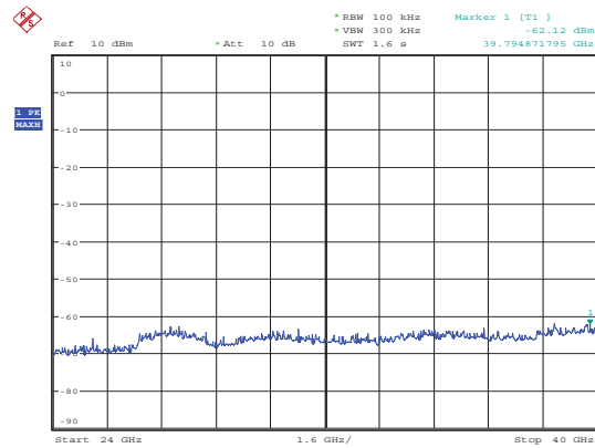
5290MHz 24GHz~40GHz
