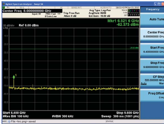
5590MHz 6.4GHz~9.6GHz
