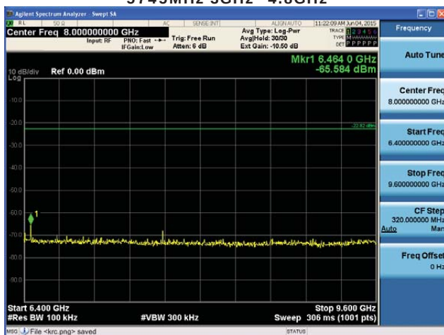
5745MHz 6.4GHz~9.6GHz
