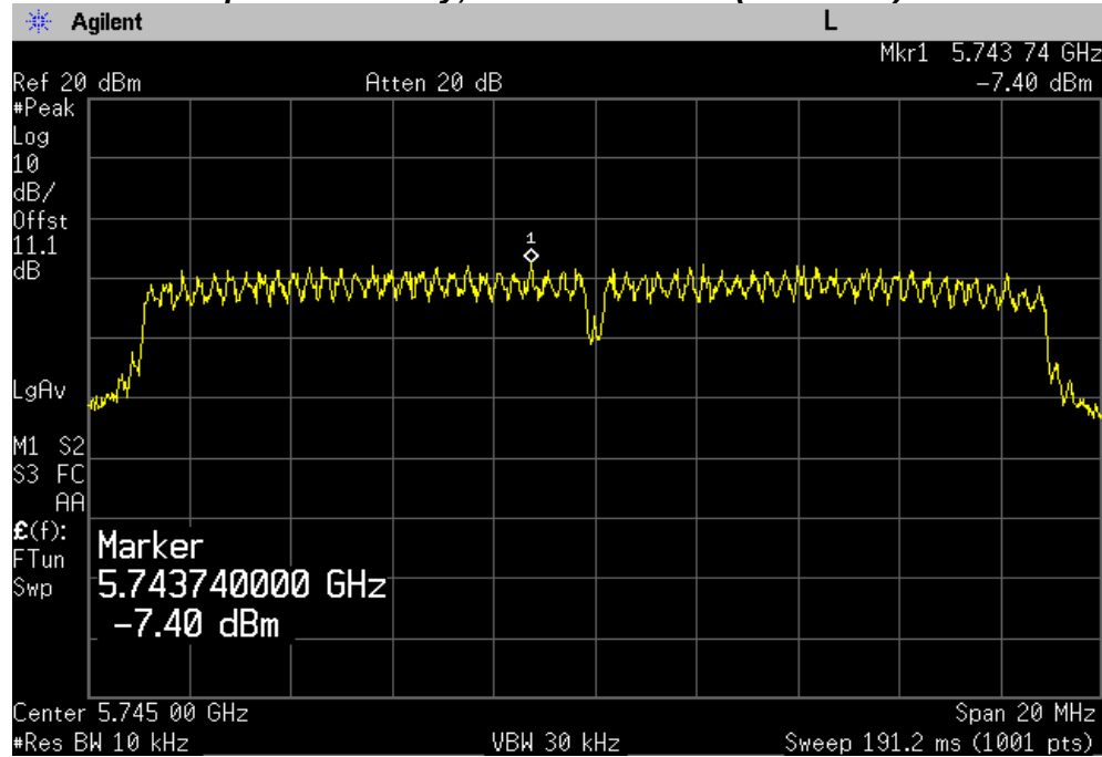
Peak Power Spectral Density, Lowest Channel (5745 MHz)
