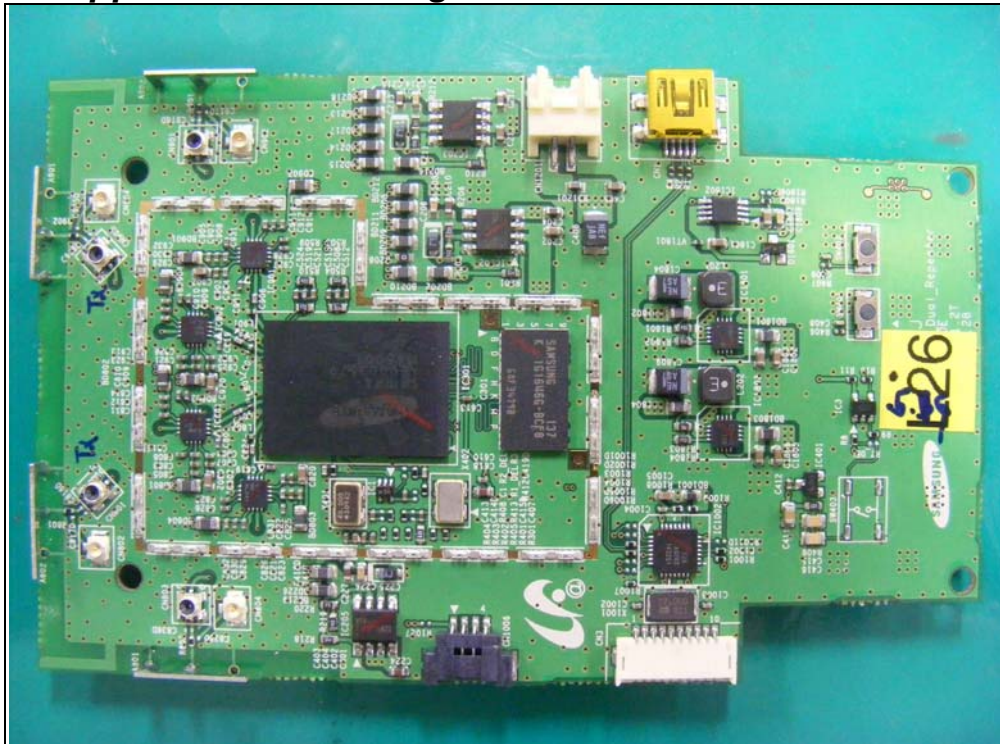
Top view of Upper PCB Removing Shield
