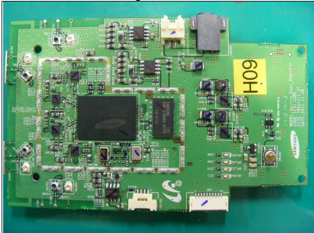
Top view of Lower PCB Removing Shield
