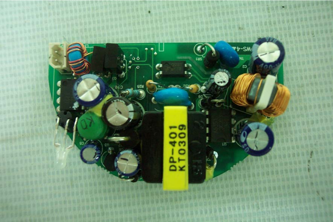
Adaptor pcb
