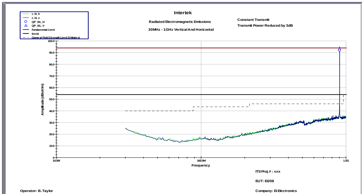
Fundamental and Spurious Emissions Below 1GHz
