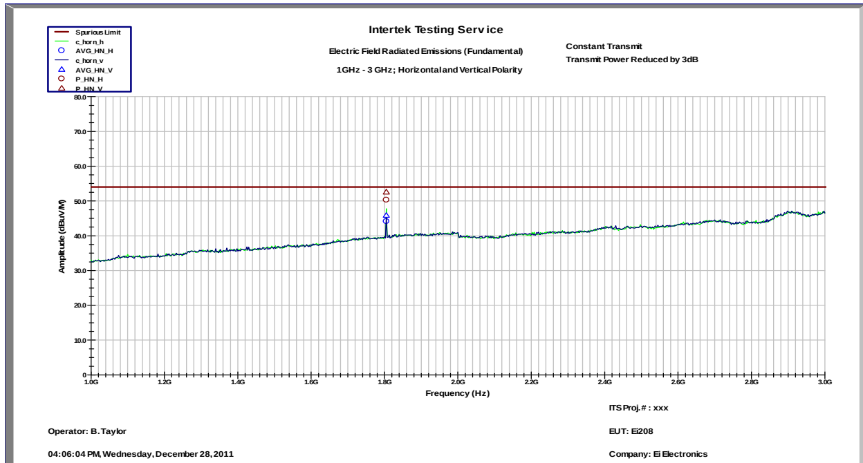
Spurious Emissions 1GHz – 3GHz
