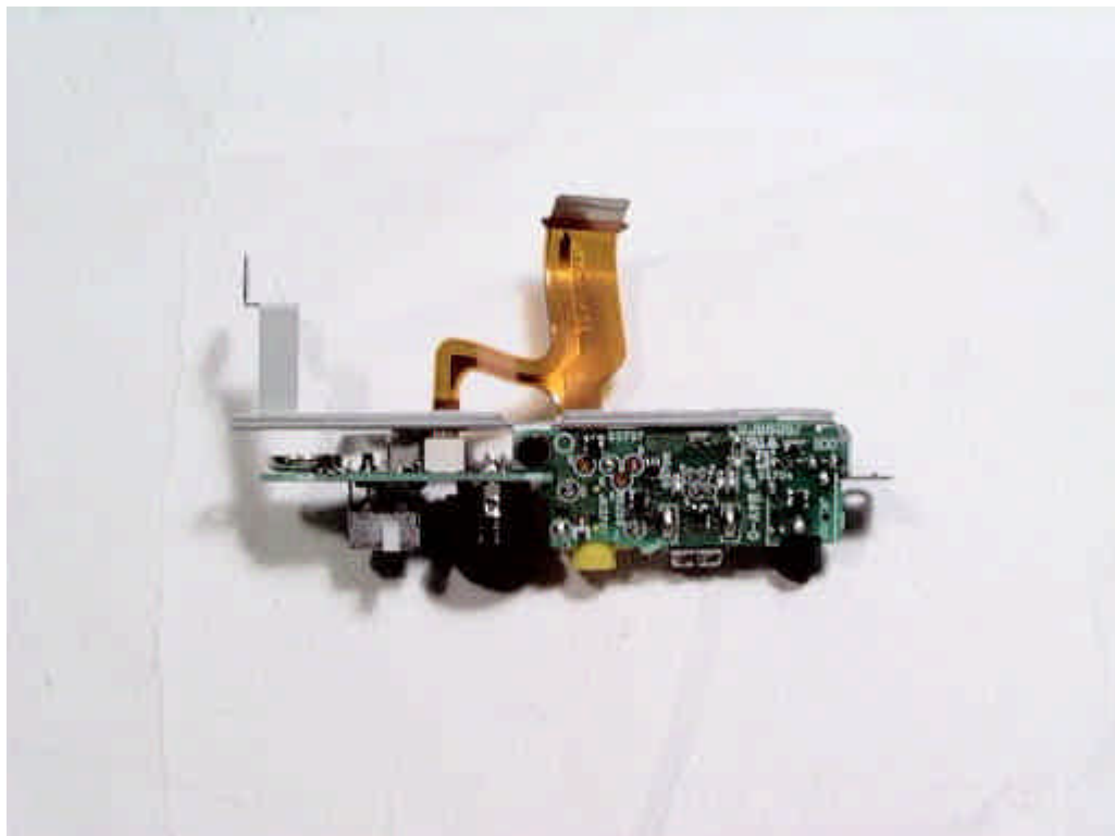
Jack PCB (Bottom view)
