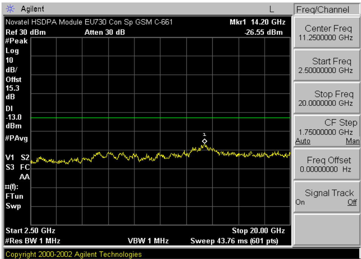
Plot A-15. Conducted Spurious Plot (PCS GPRS Mode – Ch. 661)
