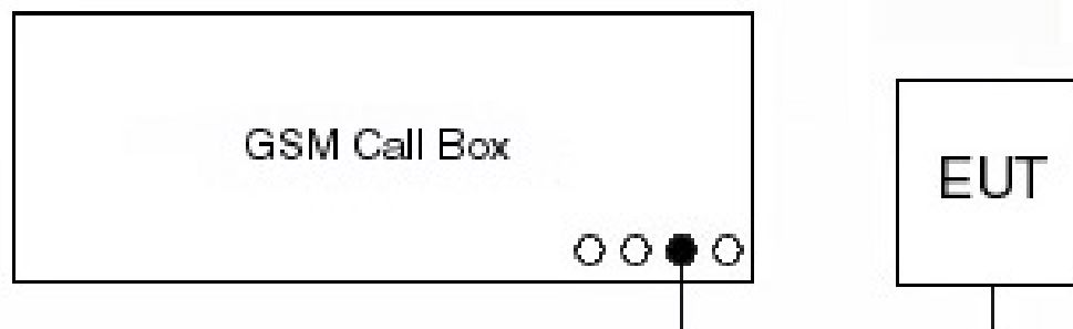
Figure 6-1. GPRS Conducted Power Test Setup Diagram
