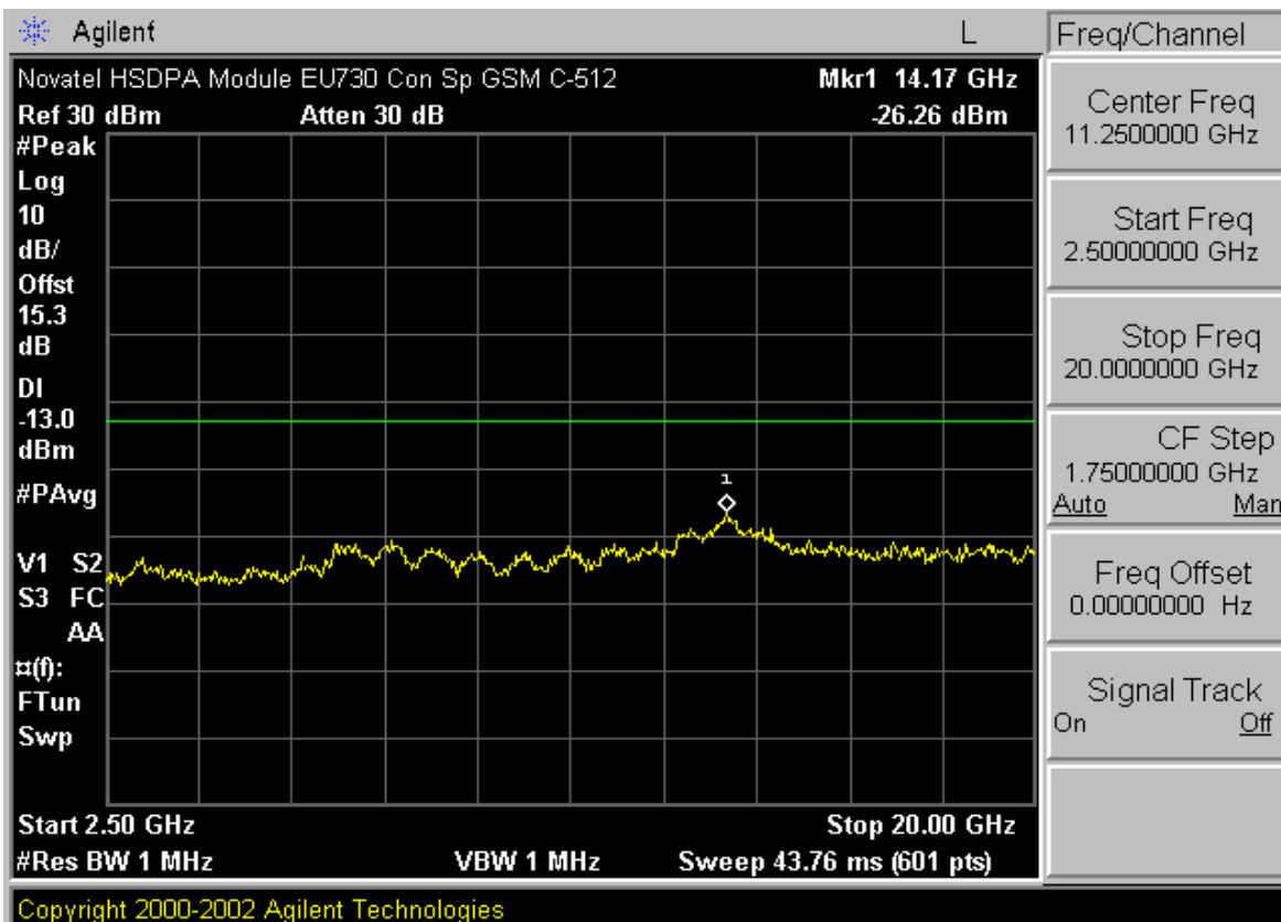
Plot A-12. Conducted Spurious Plot (PCS GPRS Mode – Ch. 512)
