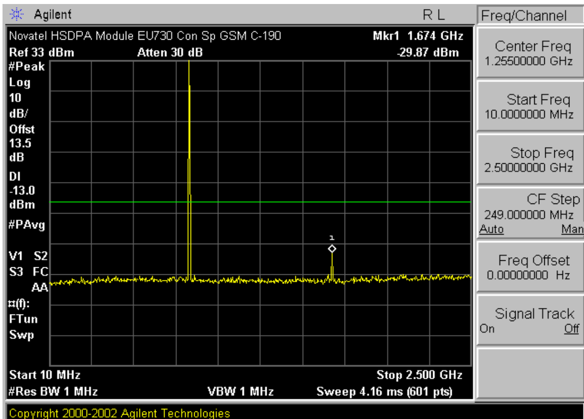
Plot A-4. Conducted Spurious (Cellular GPRS Mode – Ch. 190)
