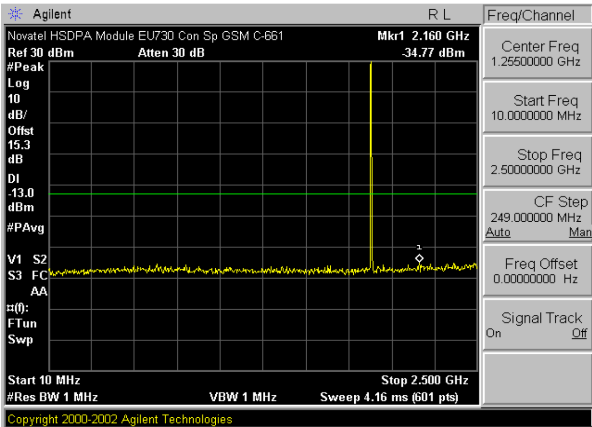
Plot A-14. Conducted Spurious Plot (PCS GPRS Mode – Ch. 661)
