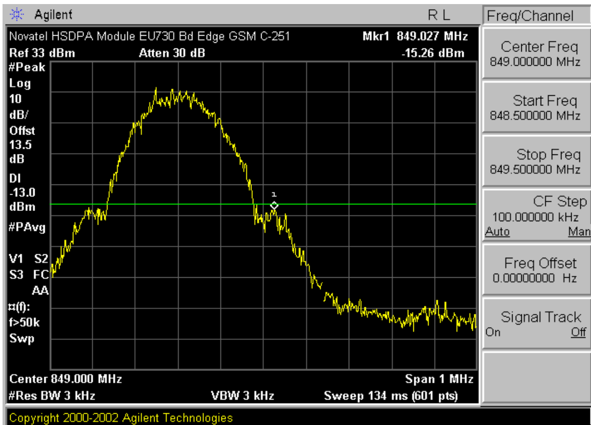
Plot A-9. Band Edge Plot (Cellular GPRS Mode – Ch. 251)
