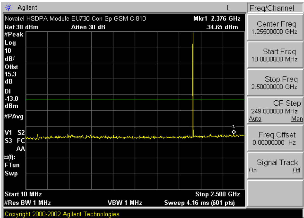
Plot A-17. Conducted Spurious Plot (PCS GPRS Mode – Ch. 810)
