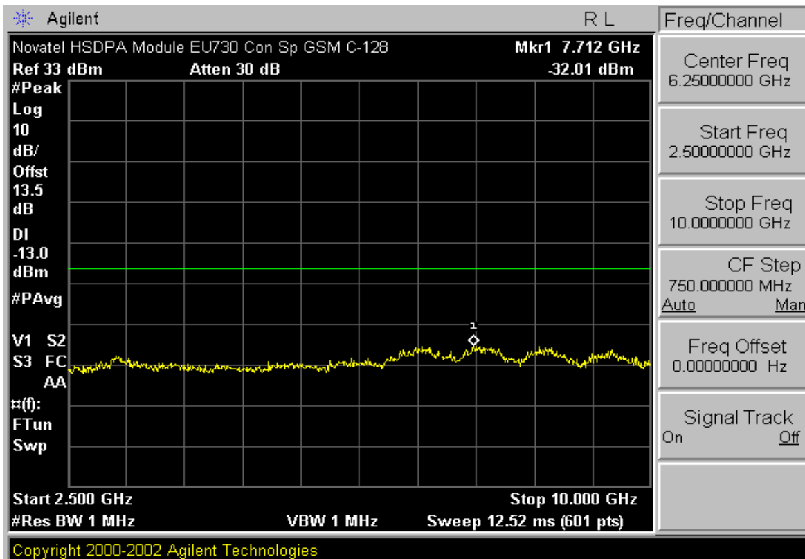
Plot A-2. Conducted Spurious Plot (Cellular GPRS Mode – Ch. 128)
