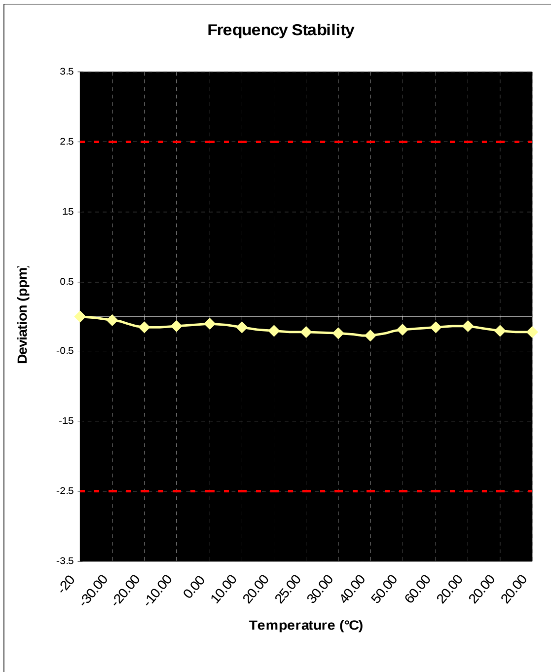
Plot 6-1. Frequency Stability Graph (Cellular GPRS Mode – Ch. 190)
