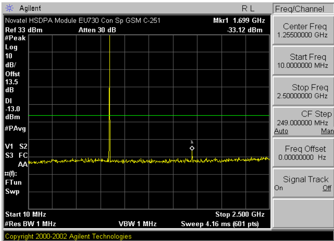
Plot A-7. Conducted Spurious Plot (Cellular GPRS Mode – Ch. 251)
