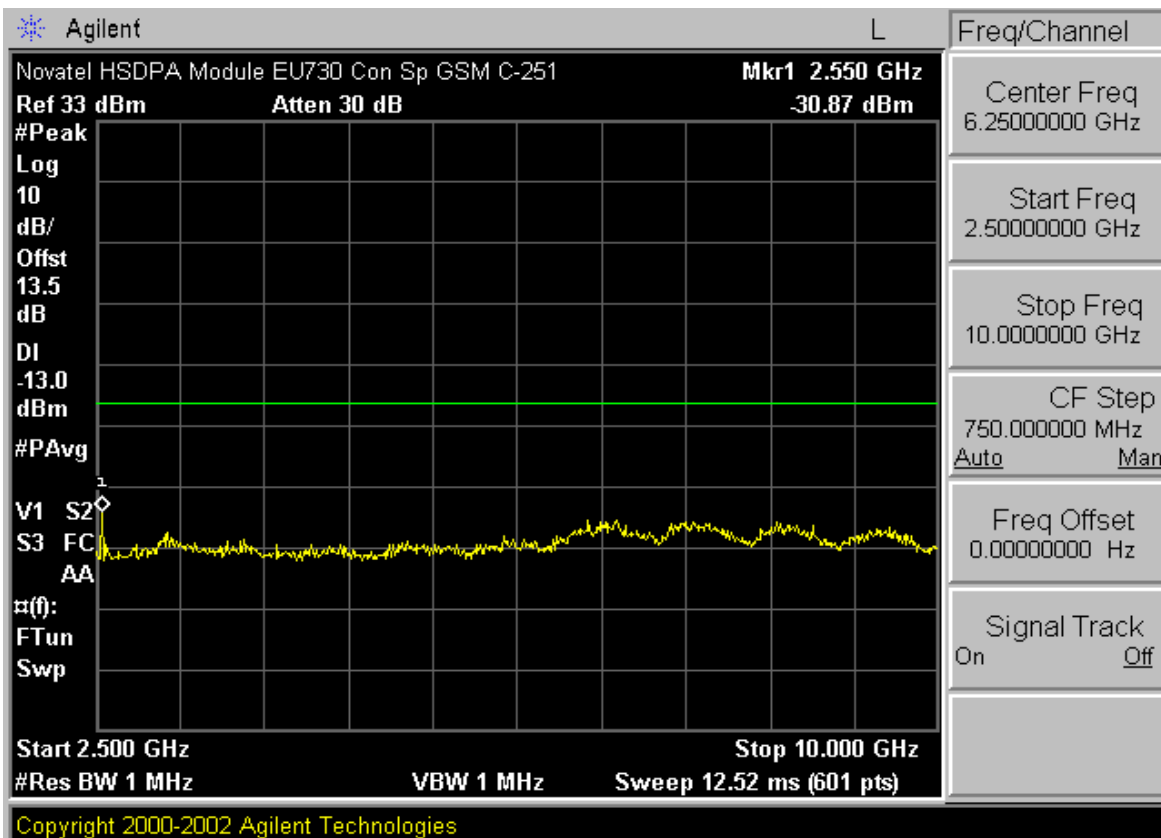
Plot A-8. Conducted Spurious Plot (Cellular GPRS Mode – Ch. 251)
