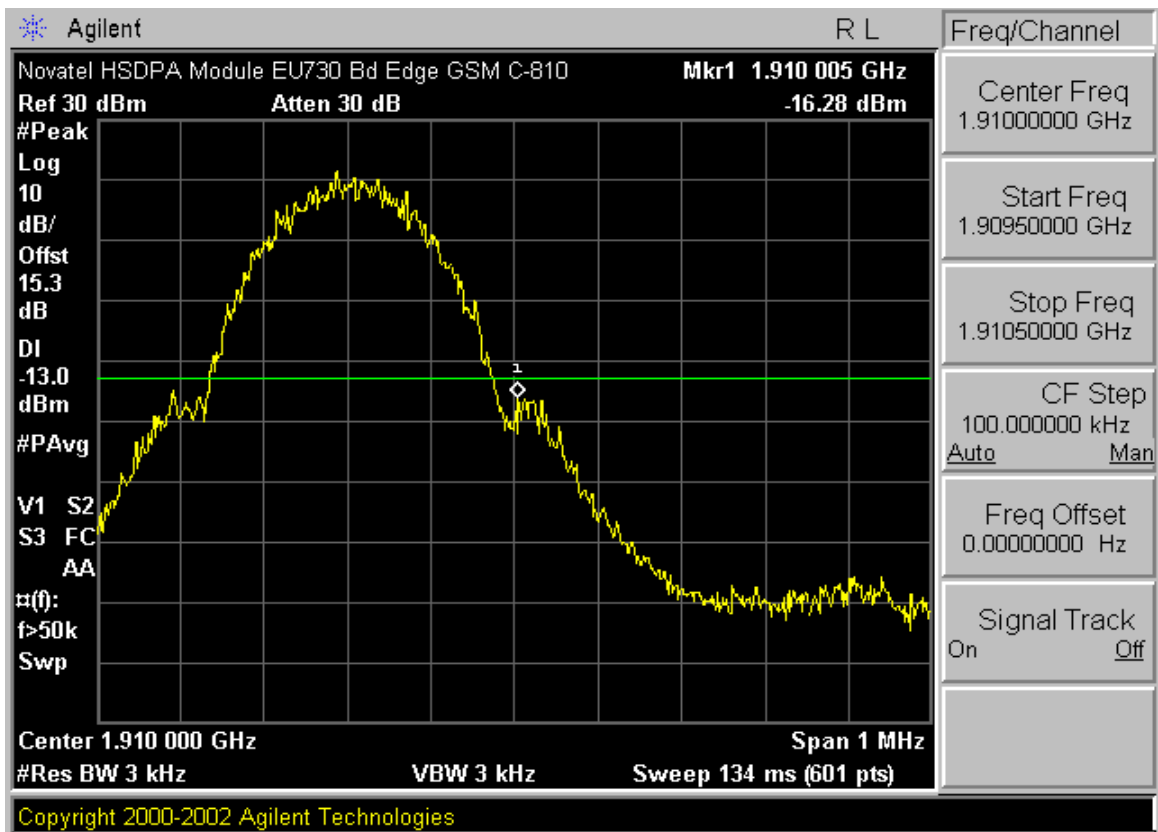
Plot A-19. Band Edge Plot (PCS GPRS Mode – Ch. 810)
