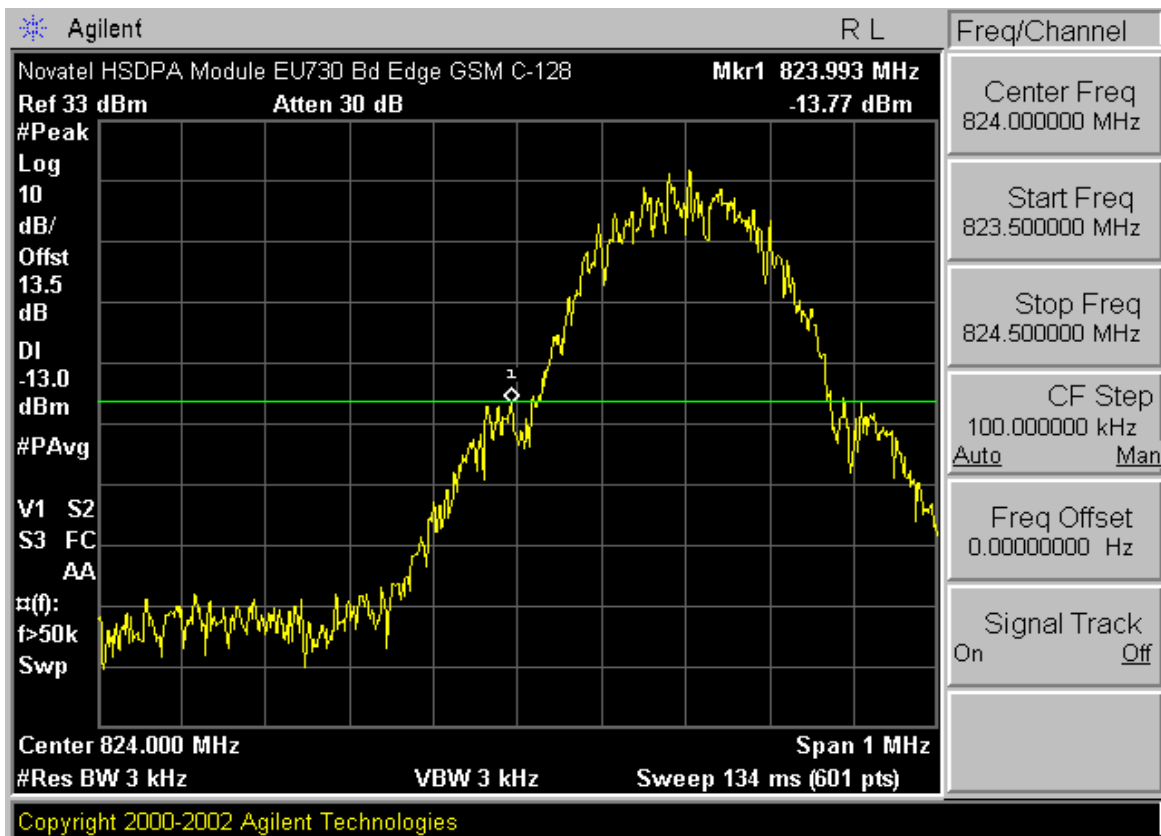
Plot A-3. Band Edge Plot (Cellular GPRS Mode – Ch. 128)
