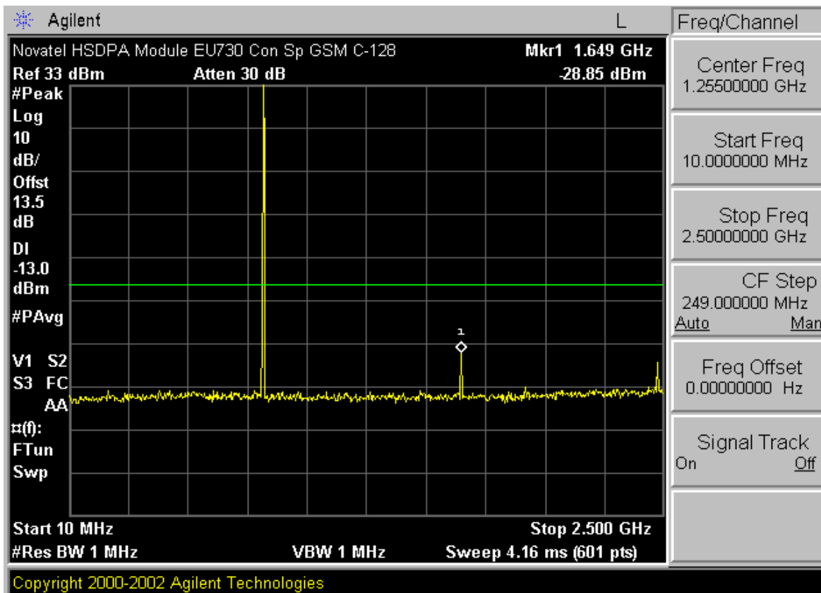
Plot A-1. Conducted Spurious Plot (Cellular GPRS Mode – Ch. 128)
