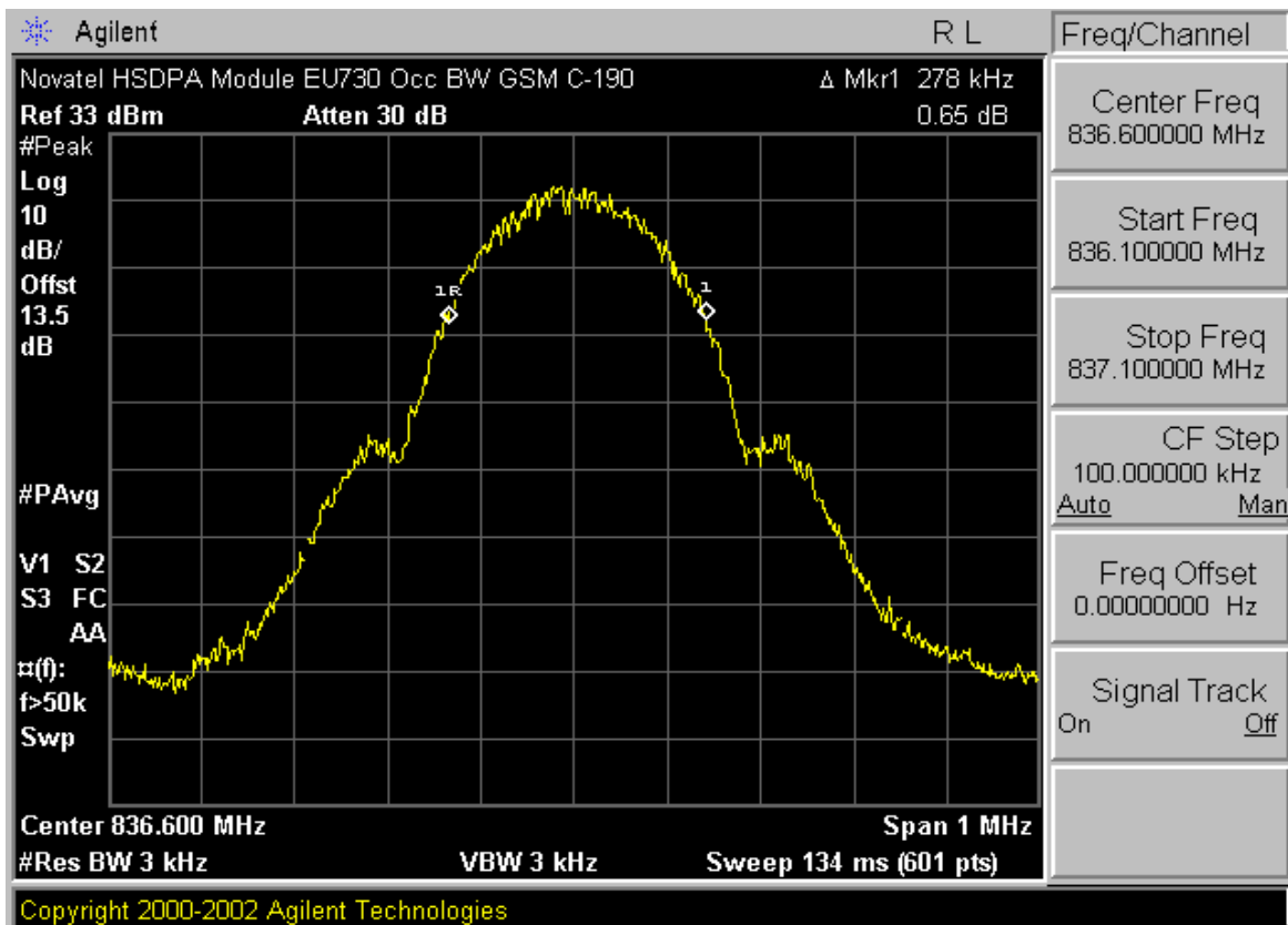
Plot A-6. Occupied Bandwidth Plot (Cellular GPRS Mode – Ch. 190)
