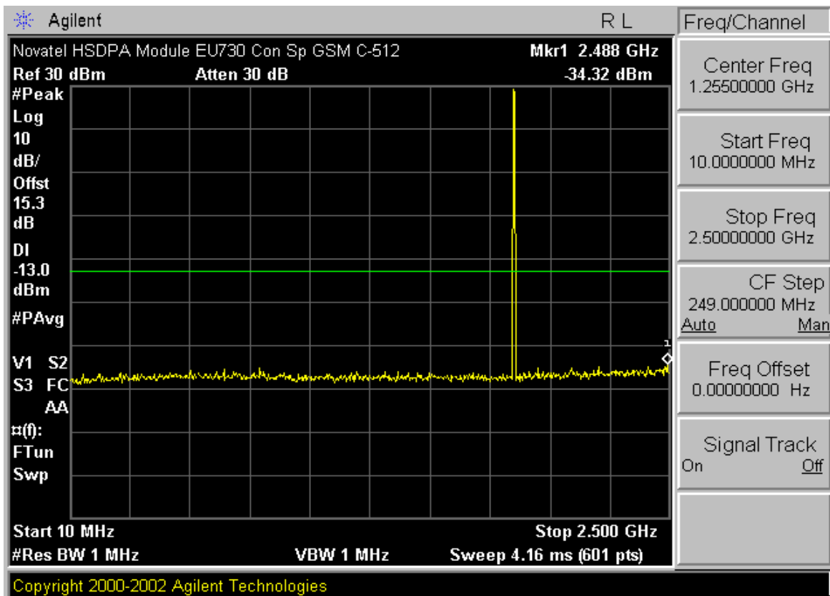
Plot A-11. Conducted Spurious Plot (PCS GPRS Mode – Ch. 512)
