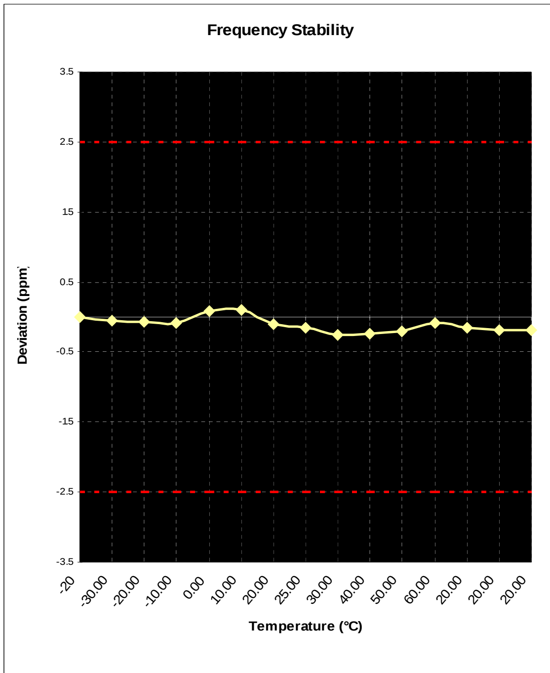
Plot 6-2. Frequency Stability Graph (PCS GPRS Mode – Ch. 661)
