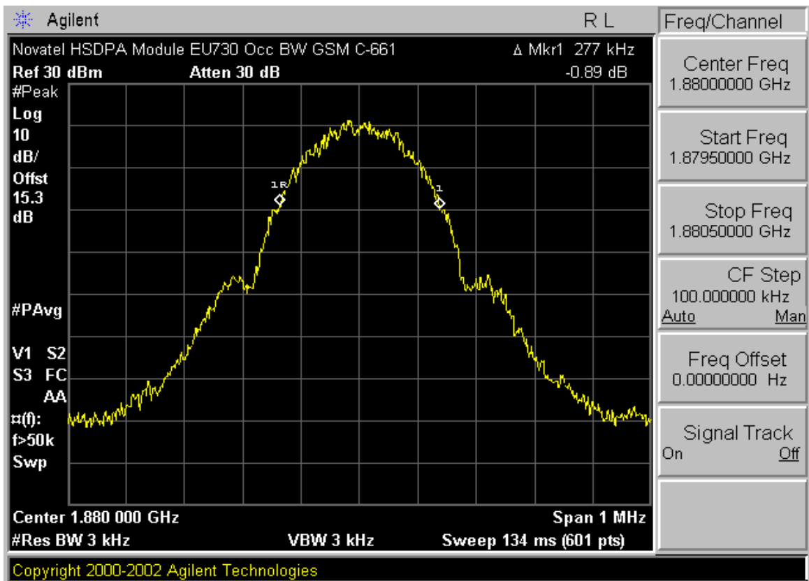
Plot A-16. Occupied Bandwidth Plot (PCS GPRS Mode – Ch. 661)
