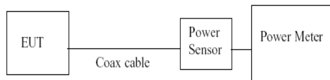
Figure 6-5. Test Instrument & Measurement Setup
