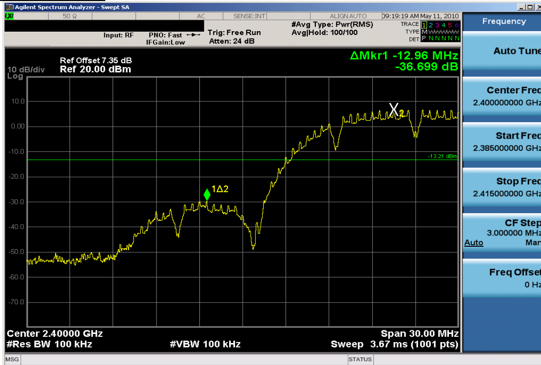
Plot 6-7. Band Edge Plot at 2Mbps (802.11b – Ch. 1)
