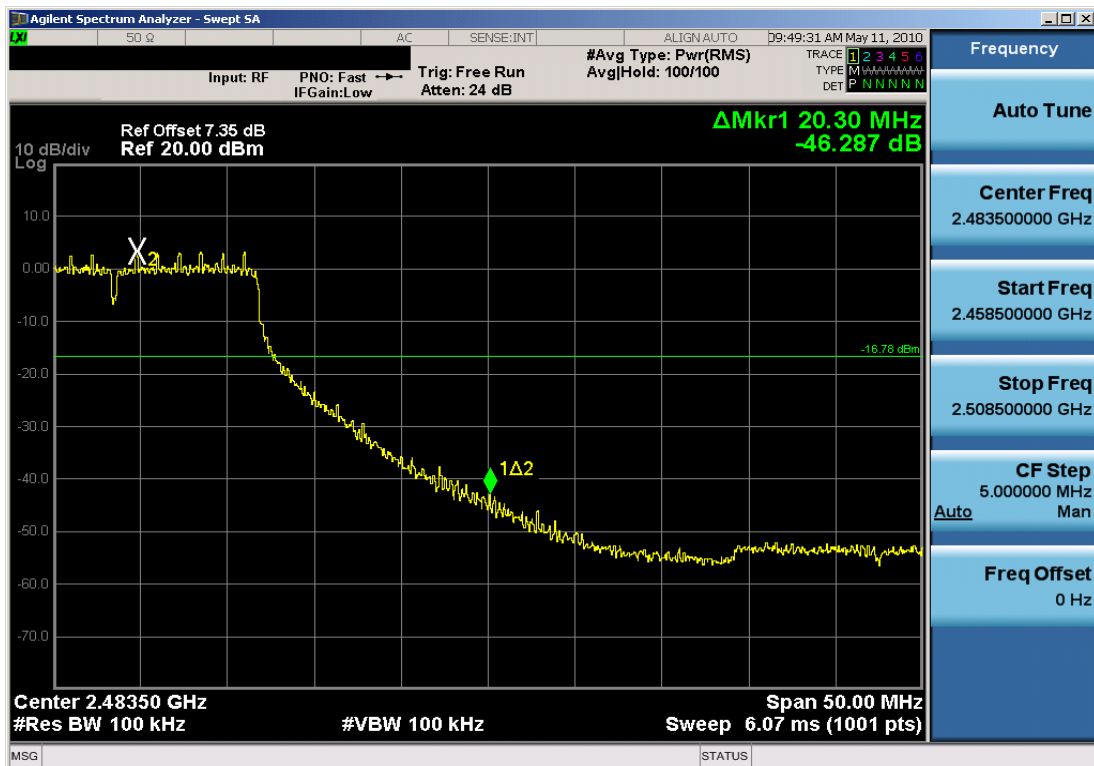
Plot 6-10. Band Edge Plot at 6Mbps (802.11g – Ch. 11)
