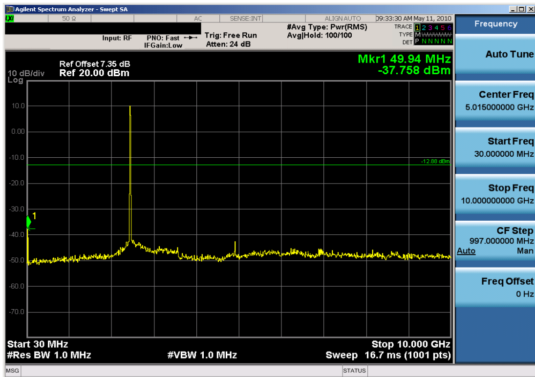
Plot 6-19. Conducted Spurious Plot at 2Mbps (802.11b – Ch. 11)
