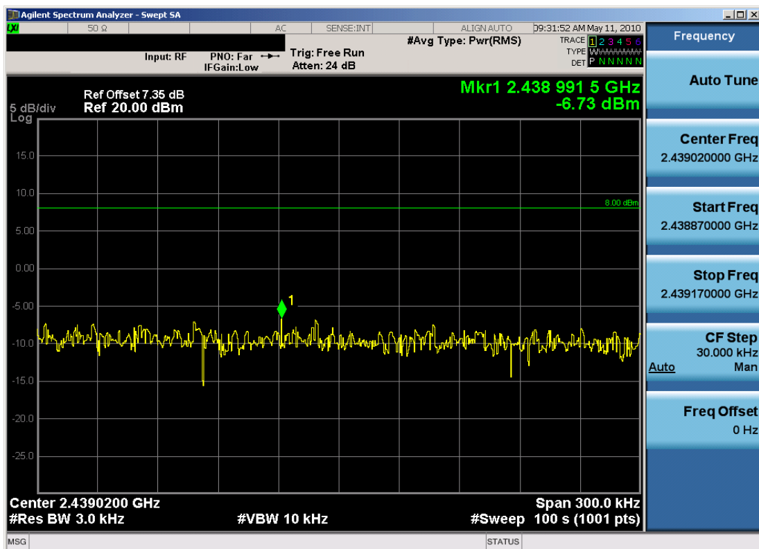
Plot 6-5. Power Spectral Density Plot at 2Mbps (802.11b – Ch. 6)
