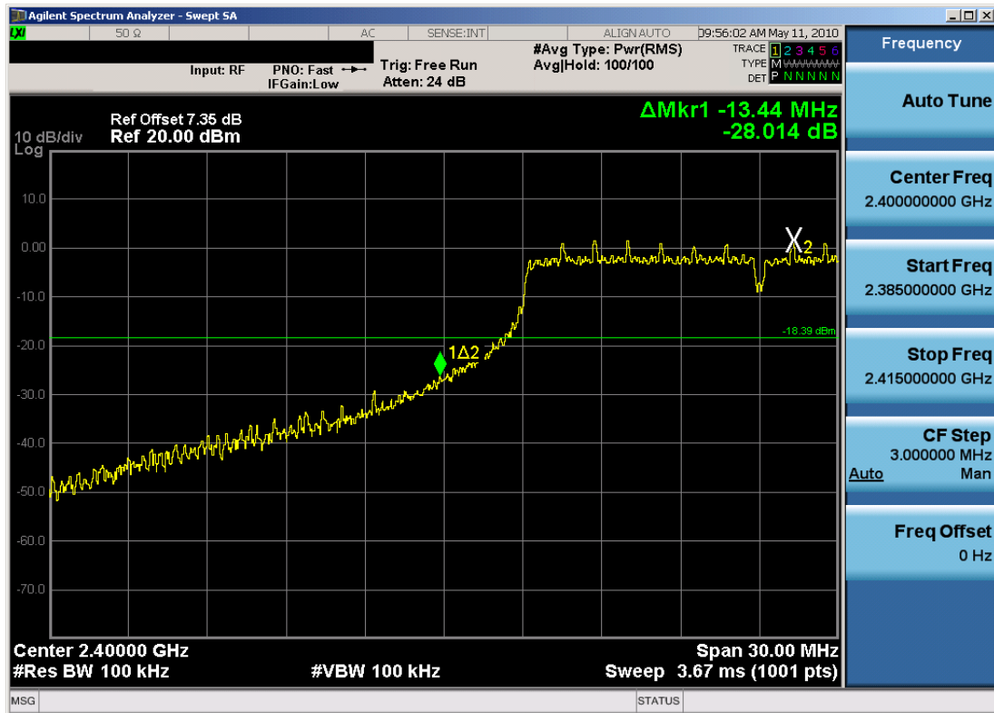
Plot 6-11. Band Edge Plot at 6.5Mbps (MCS0) (802.11n – Ch. 1)
