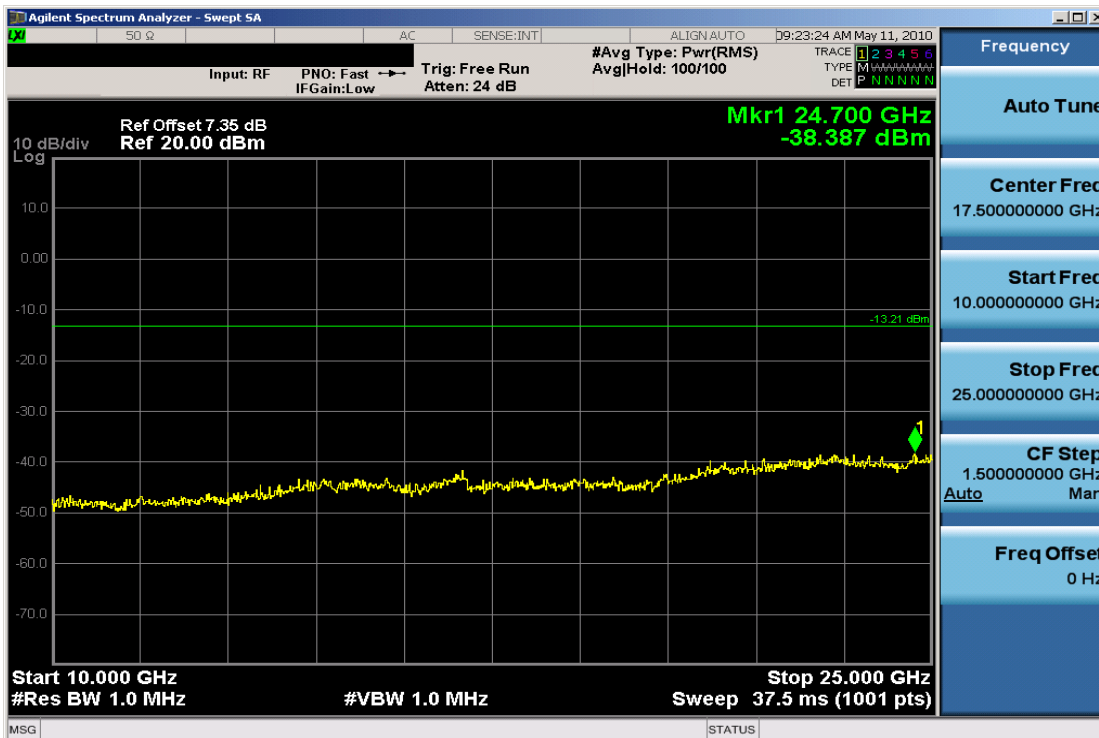
Plot 6-16. Conducted Spurious Plot at 2Mbps (802.11b – Ch. 1)
