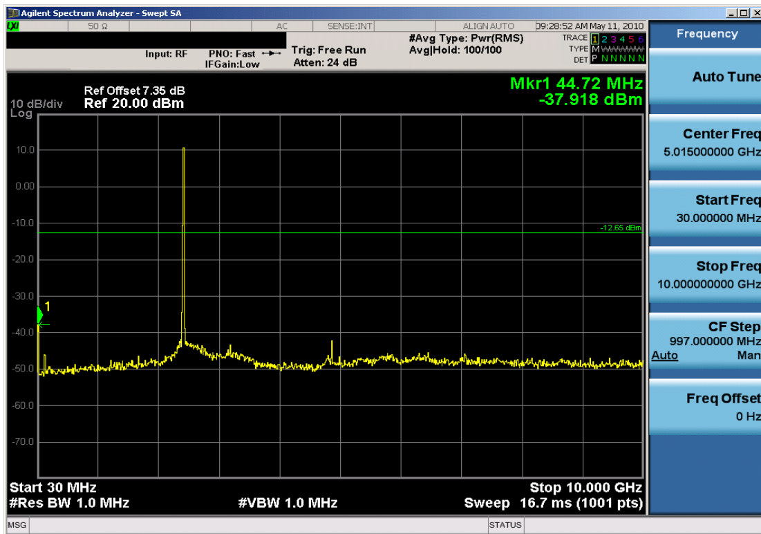
Plot 6-17. Conducted Spurious Plot at 2Mbps (802.11b – Ch. 6)
