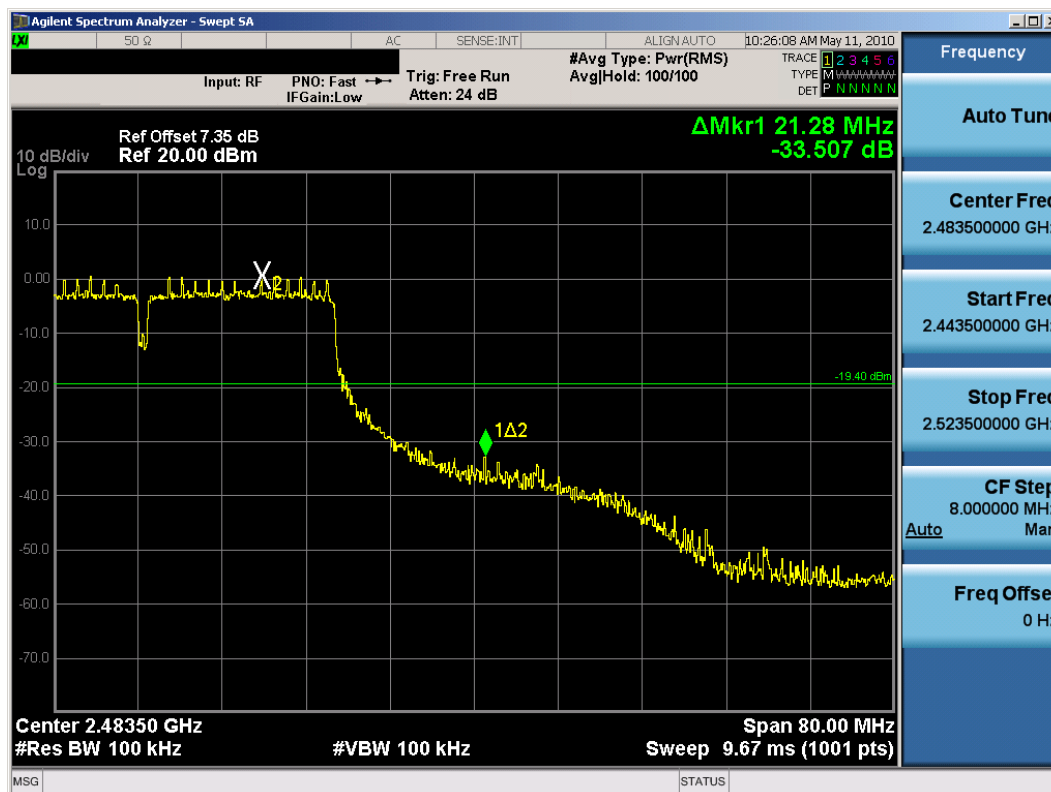
Plot 6-14. Band Edge Plot at 81Mbps (MCS4) (802.11n (40MHz) – Ch. 9)
