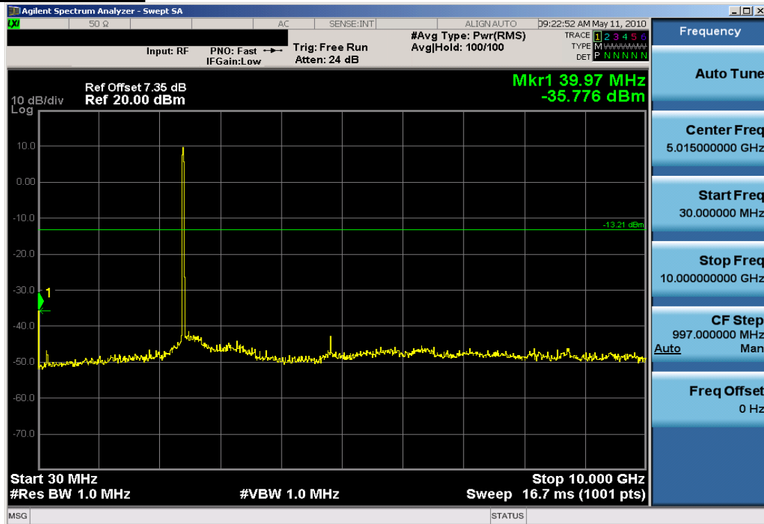
Plot 6-15. Conducted Spurious Plot at 2Mbps (802.11b – Ch. 1)
