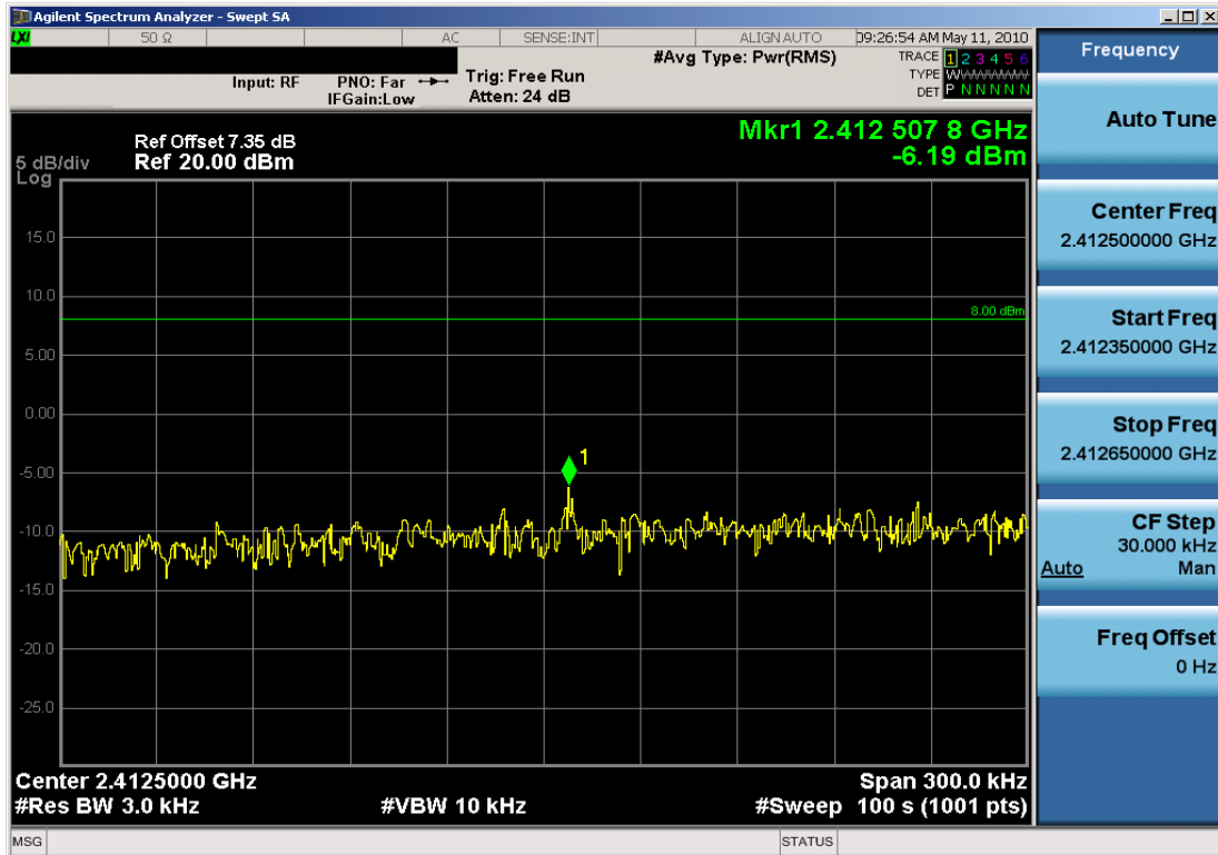
Plot 6-4. Power Spectral Density Plot at 2Mbps (802.11b – Ch. 1)
