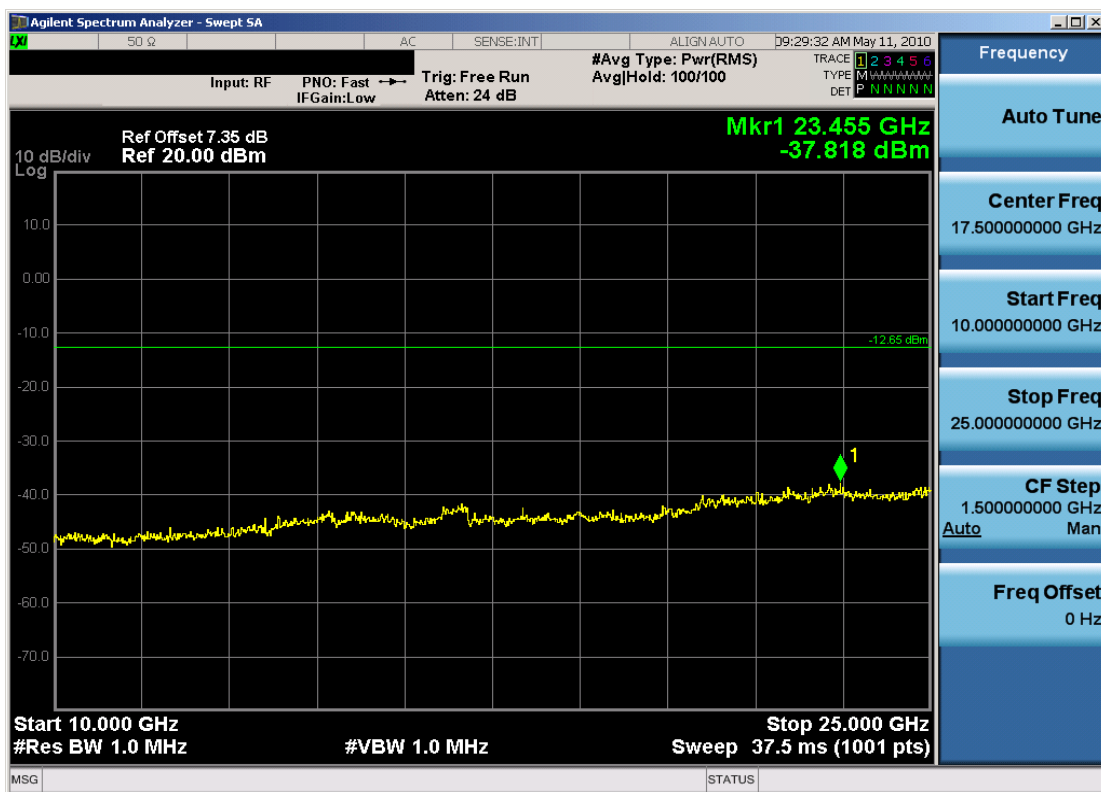
Plot 6-18. Conducted Spurious Plot at 2Mbps (802.11b – Ch. 6)
