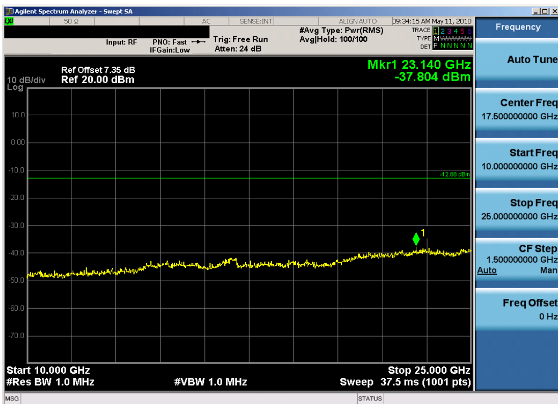
Plot 6-20. Conducted Spurious Plot at 2Mbps (802.11b – Ch. 11)
