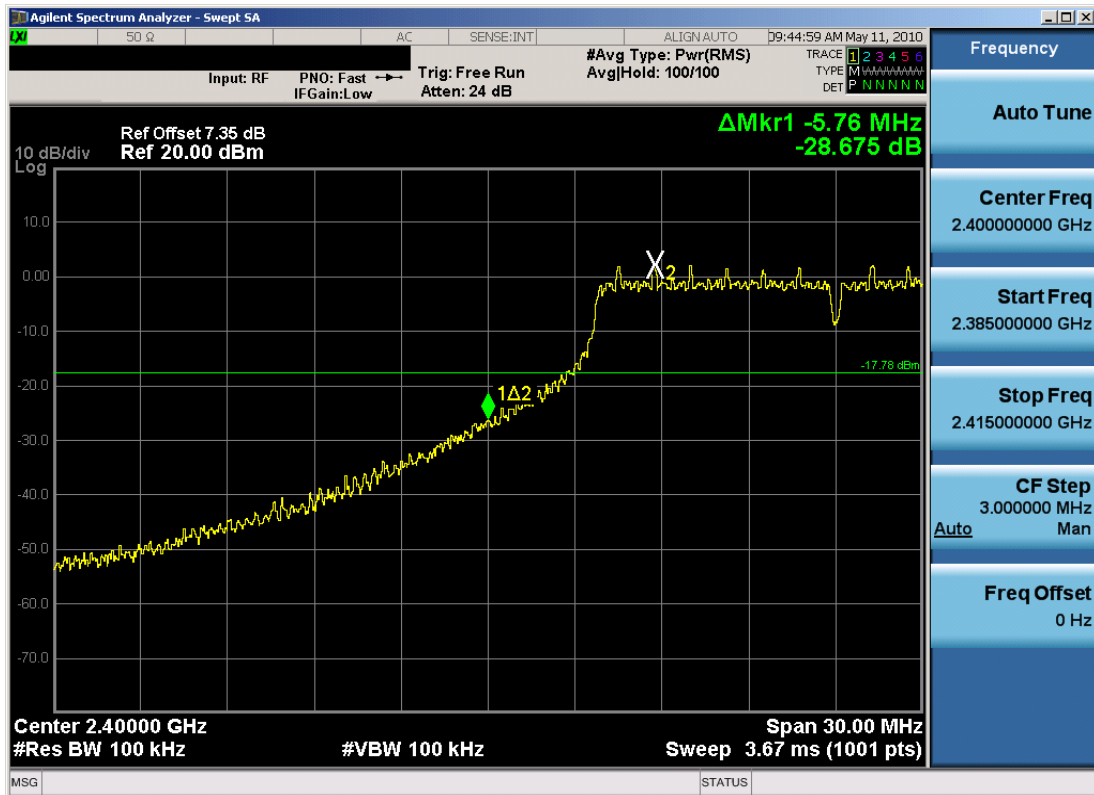
Plot 6-9. Band Edge Plot at 6Mbps (802.11g – Ch. 1)
