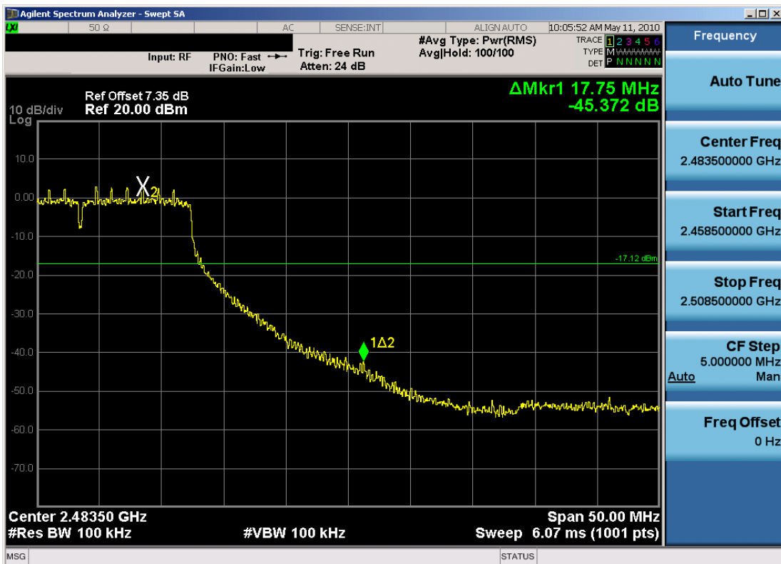
Plot 6-12. Band Edge Plot at 6.5Mbps (MCS0) (802.11n – Ch. 11)
