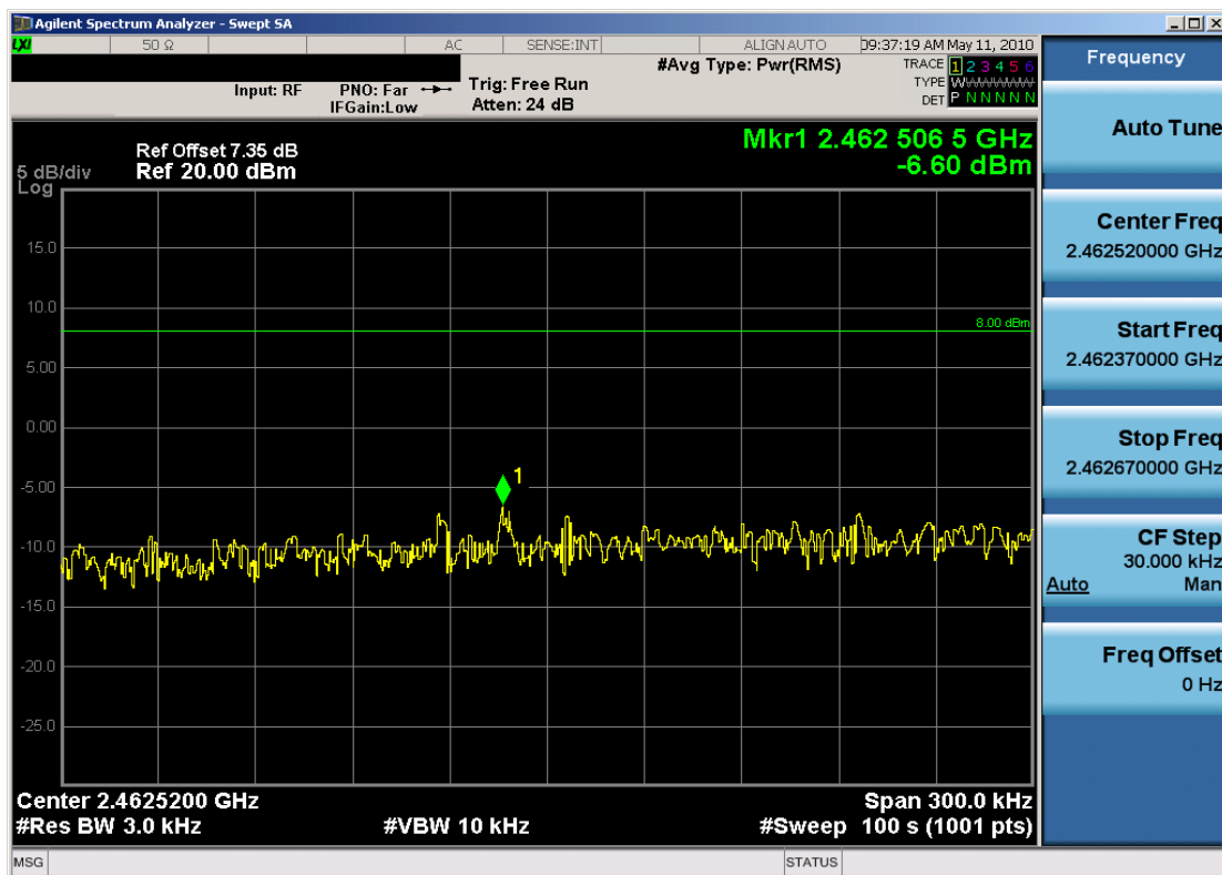
Plot 6-6. Power Spectral Density Plot at 2Mbps (802.11b – Ch. 11)
