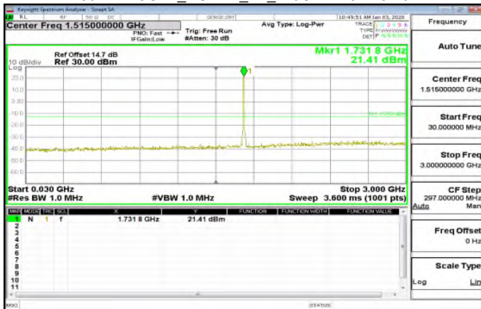
30MHz~3GHz_HSDPA_B4_MidCH1413-1732.6
