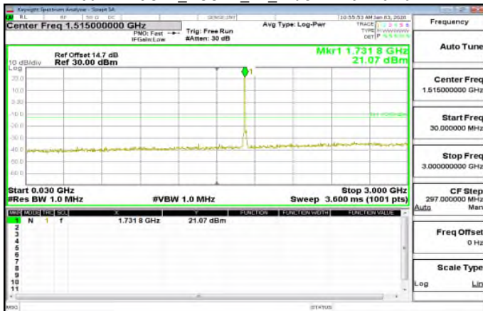
30MHz~3GHz_HSUPA_B4_MidCH1413-1732.6
