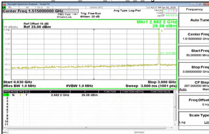
30MHz~3GHz_Band41_10MHz_QPSK_1_0_HighCH41540-2685
