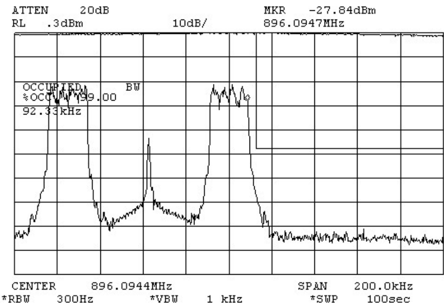
Figure 6-83: WIDEN50 Split Quad-QPSK Modulation performance relative to mask 47 CFR 90.669(a) (MAXIMUM POWER SETTING)
