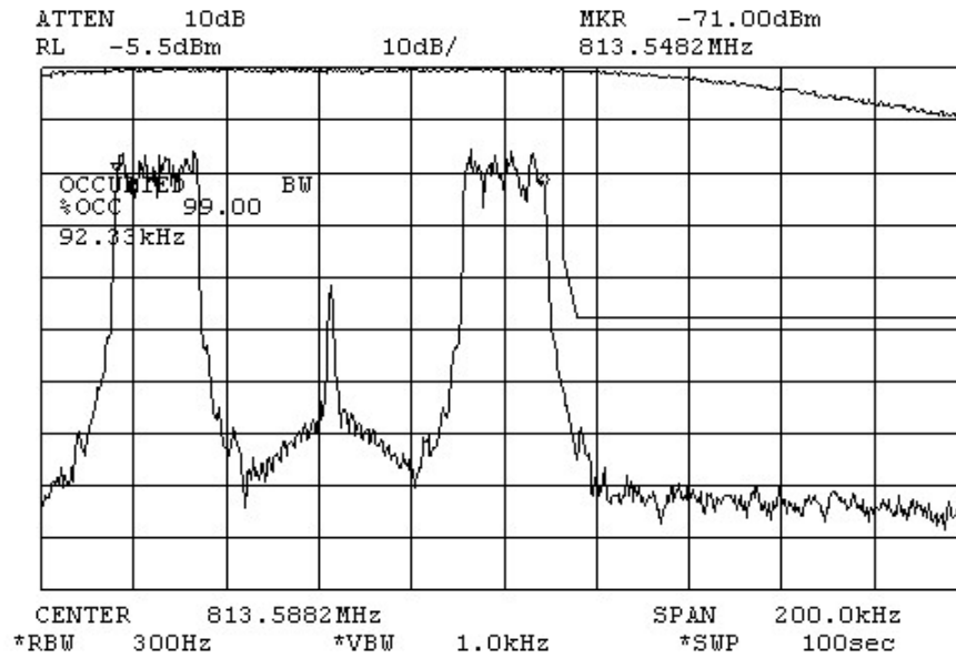
Figure 6-53: WiDEN50 Split Quad-QPSK Modulation performance relative to mask 47 CFR 90.691. (MAXIMUM POWER SETTING)
