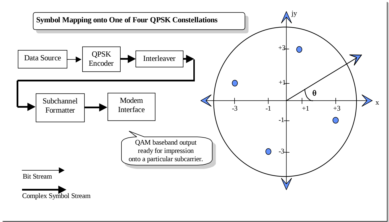
Figure 6-3: Symbol Mapping onto One of Four QPSK Constellations
