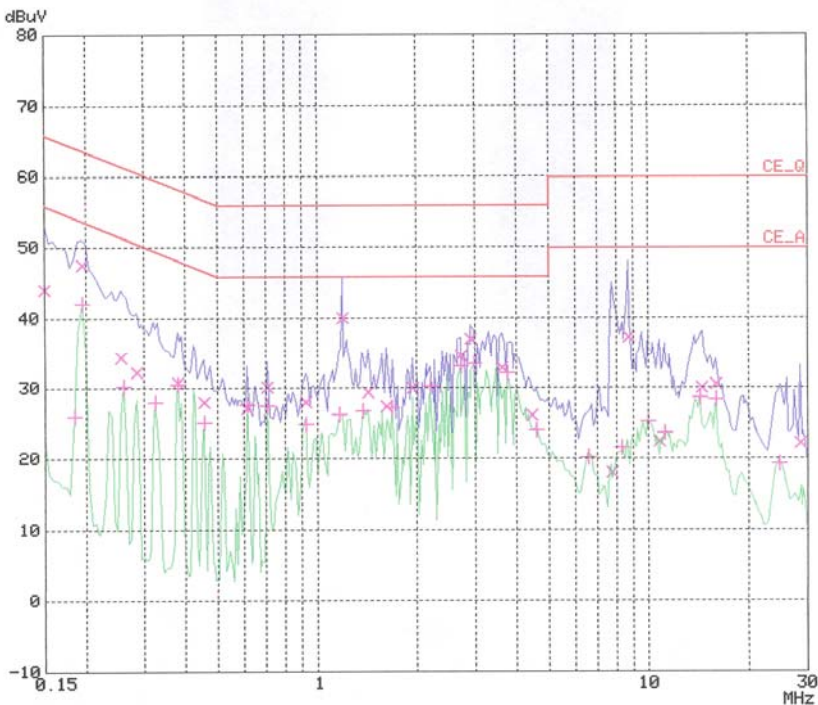
< Neutral line >
