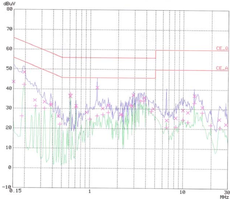
< Hot line >
