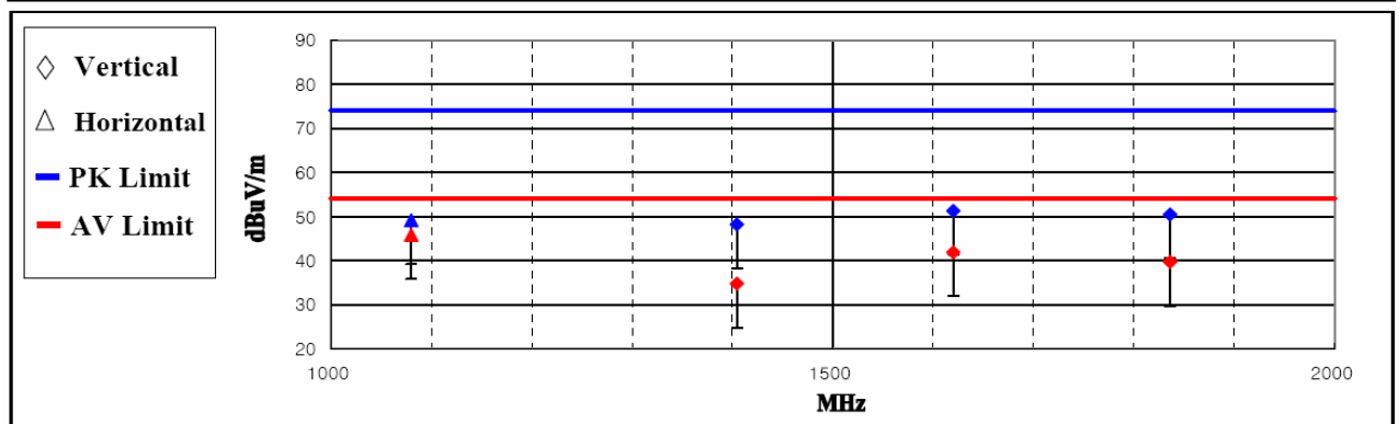
&lt; Fig 7. Radiated emission result (1000MHz ~ 2000MHz)&gt;
