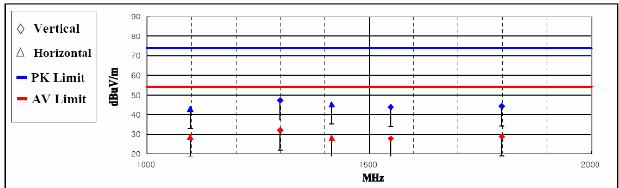
&lt; Fig 6. Radiated emission result (1000MHz ~ 2000MHz)&gt;
