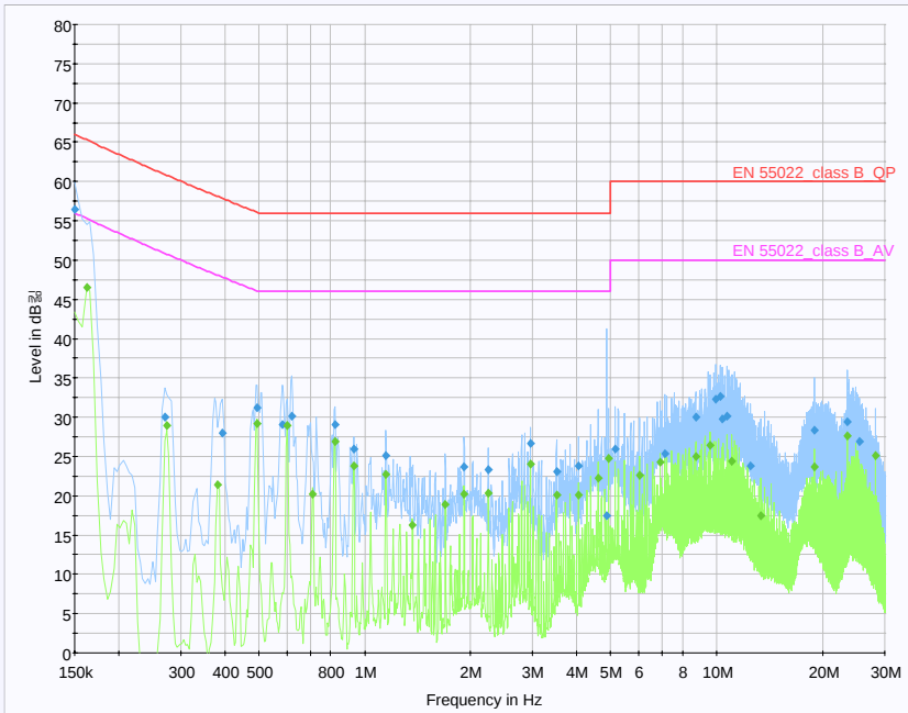
< Hot line >
