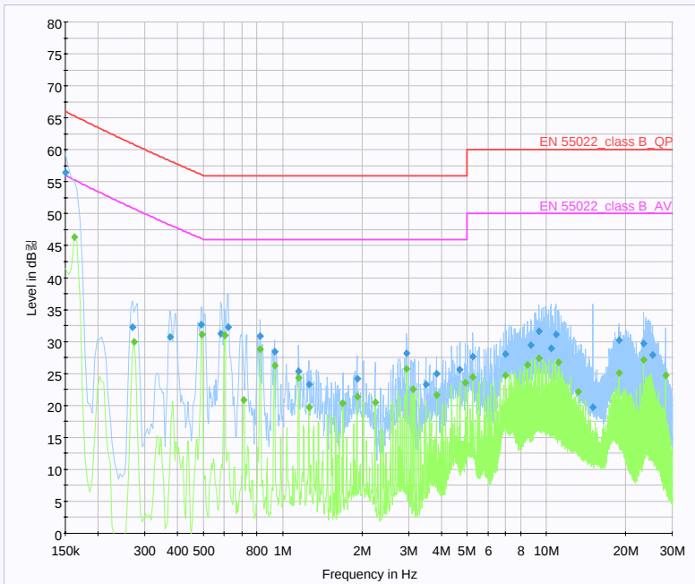
< Neutral line >
