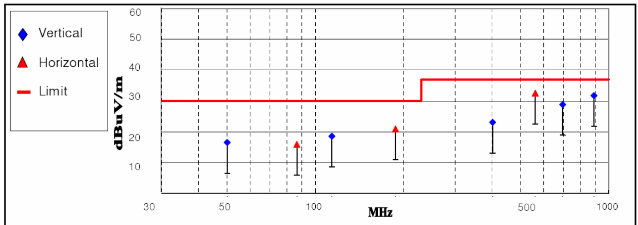
< Fig 4. Radiated emission result _ Analog >
