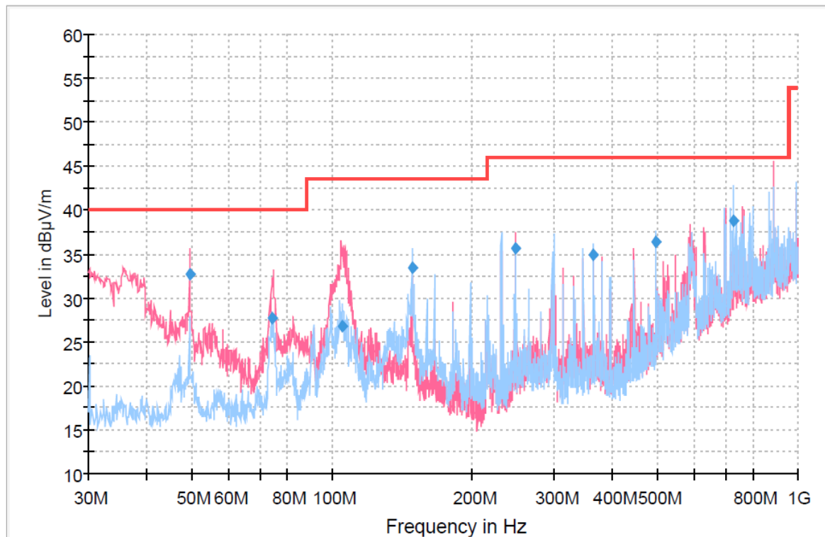
RE_below 1GHz
