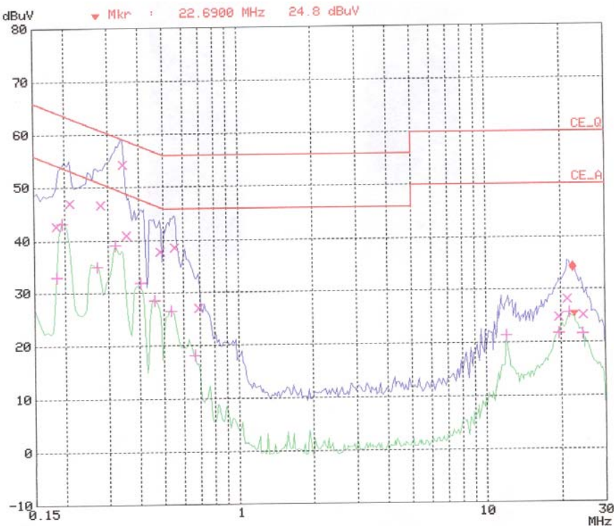
< Hot line >
