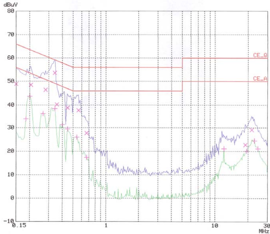
< Neutral line >
