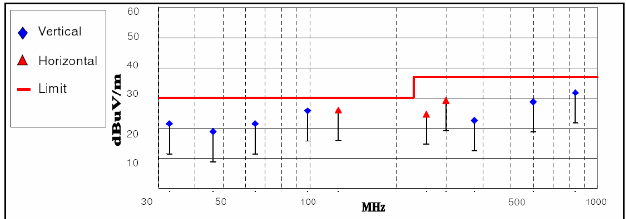
< Fig 5. Radiated emission result _ Digital >
