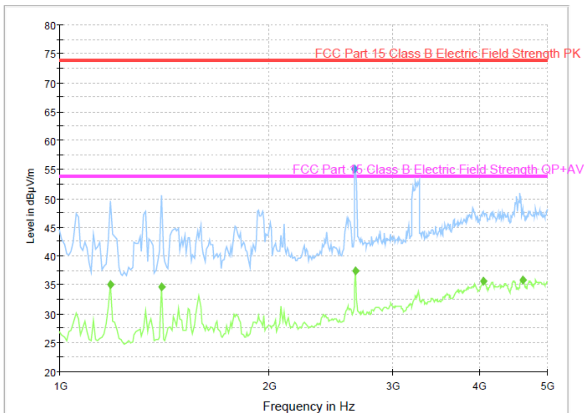
Radiated Emission_above 1 GHz
