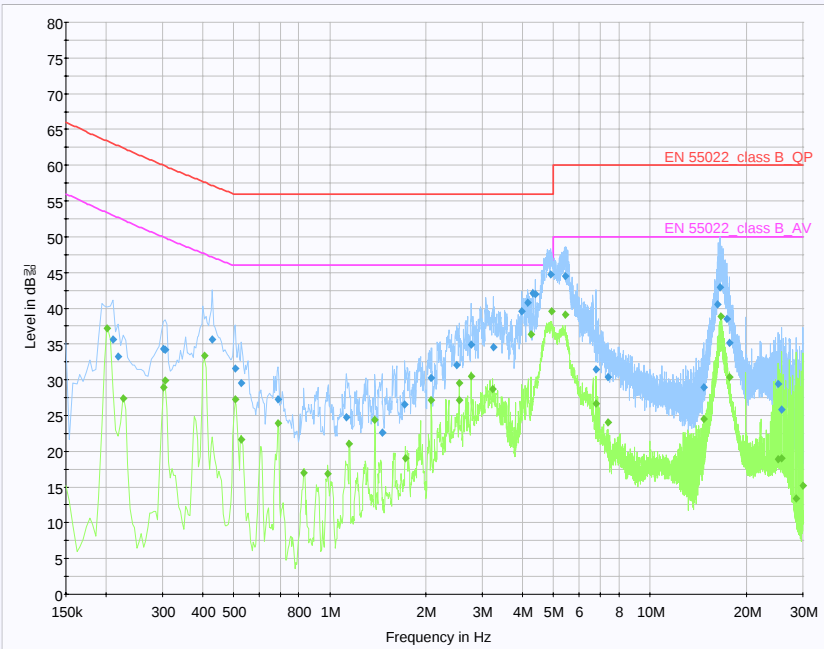
< Hot line >
