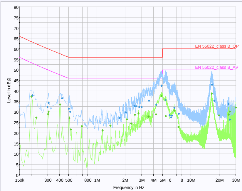
< Neutral line >
