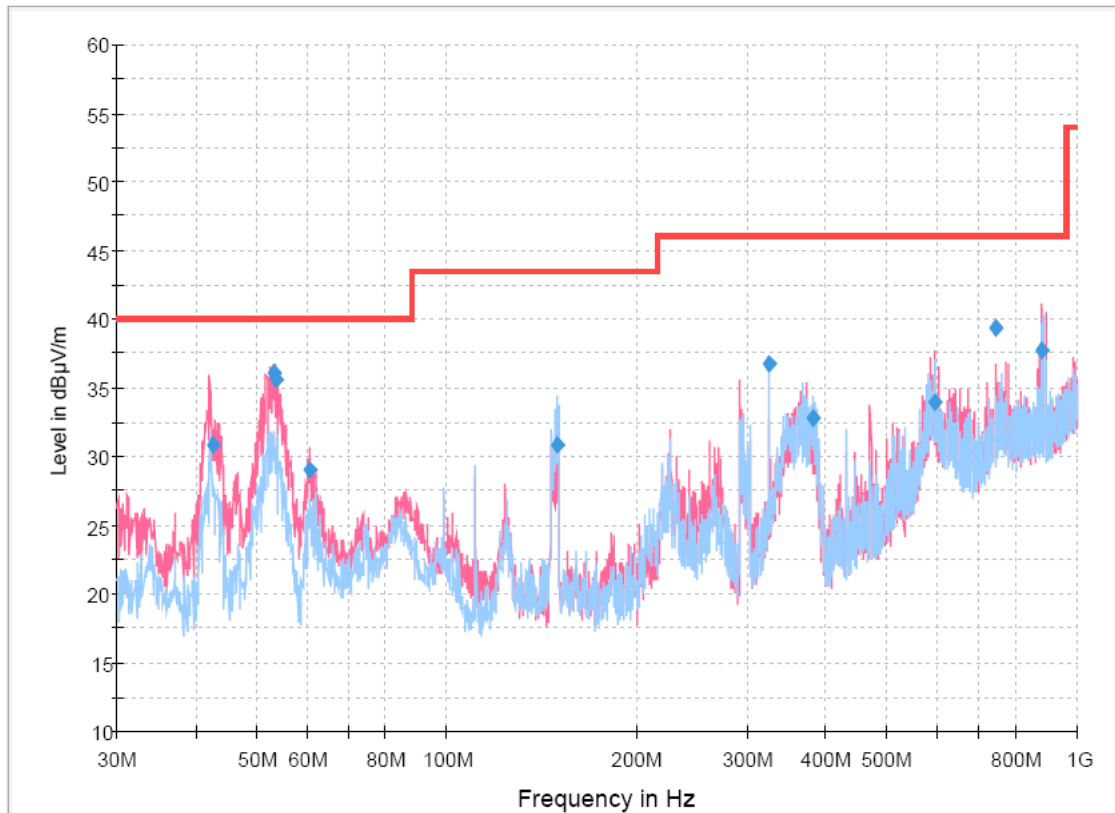
RE_below 1GHz
