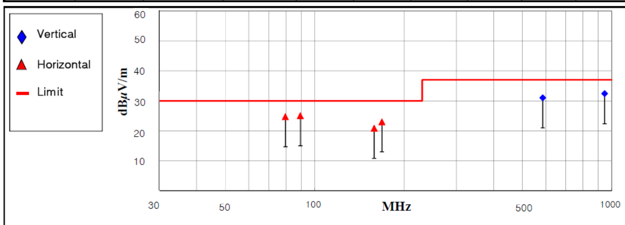
< Fig 13. Radiated emission result (30 MHz ~ 1 000 MHz) >
