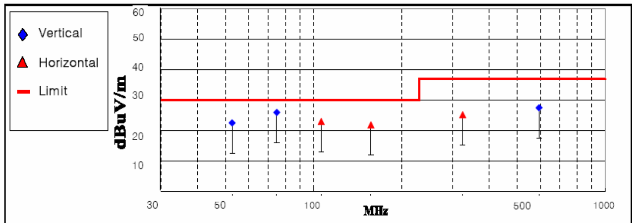
< Fig 4. Radiated emission result _ Digital >
