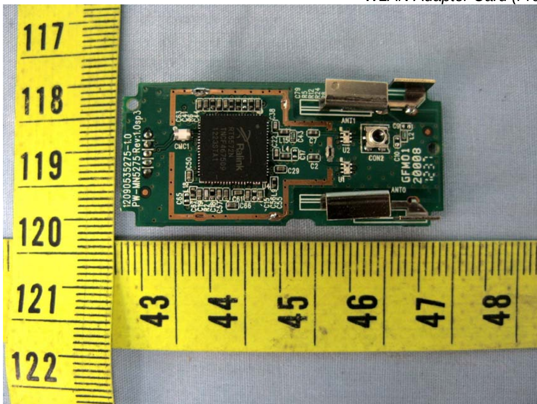
Figure 2 WLAN Adapter Card (Front View)
