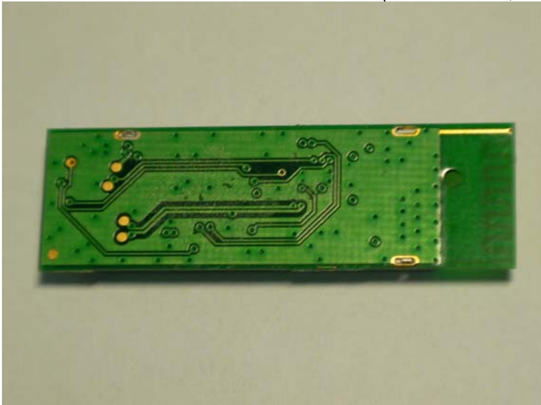
Figure 23 Internal View (Bluetooth Module, Back View)
