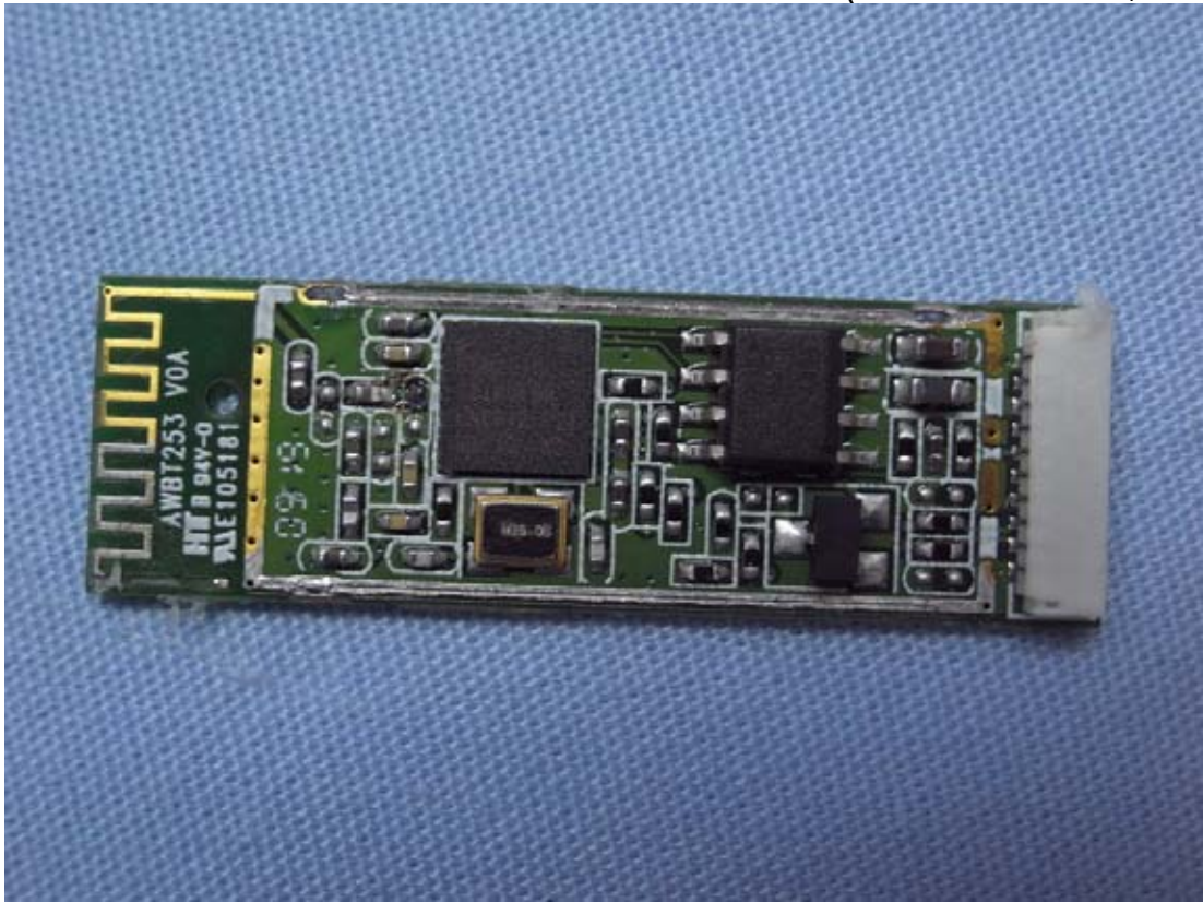
Figure 21 Internal View (Bluetooth Module, Front View)
