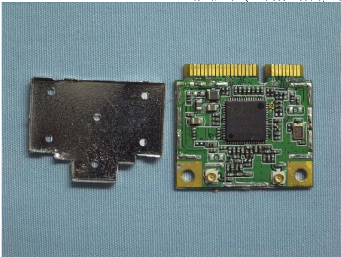
Figure 17 Internal View (Wireless Module, Front View)
