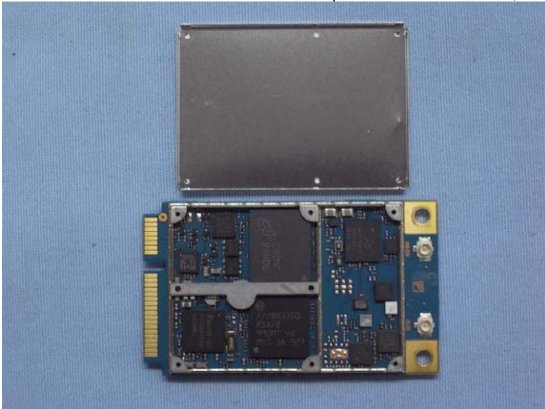
Figure 25 Internal View (Mobil Broadband Module, Front View)
