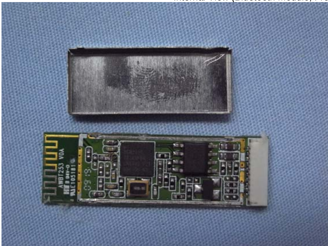
Figure 20 Internal View (Bluetooth Module, Front View)
