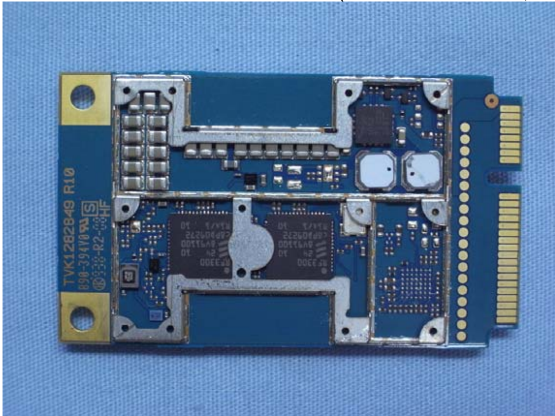
Figure 27 Internal View (Mobil Broadband Module, Back View)
