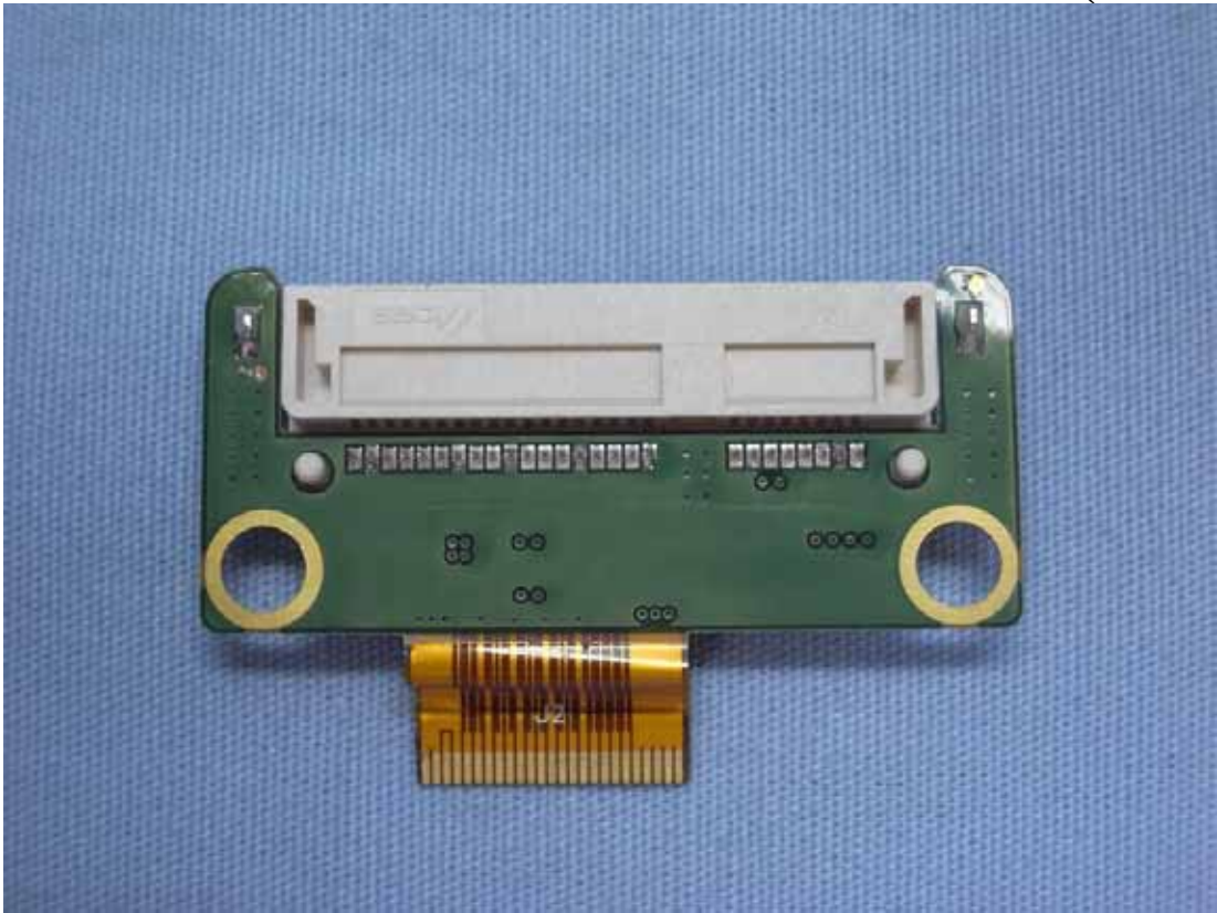
Figure 16 Connect Board (Back View)
