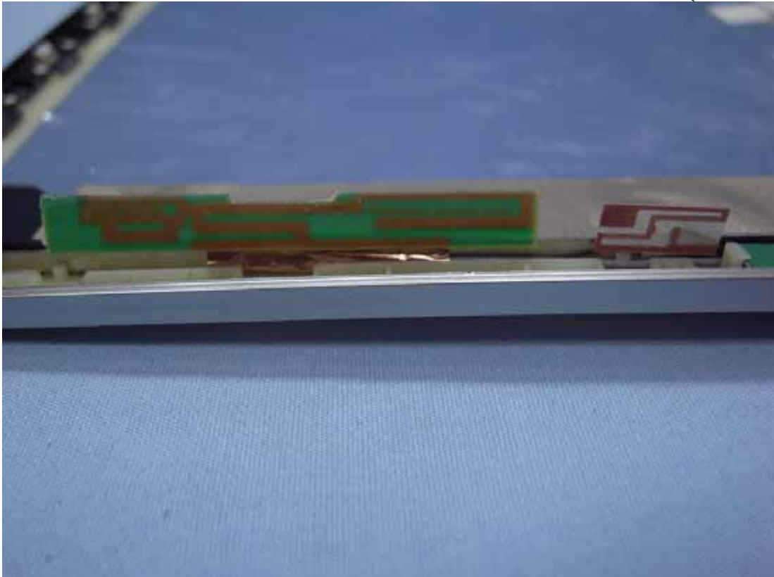
Figure 43 Mobil Broadband & Wireless LAN Antenna (Front View)
