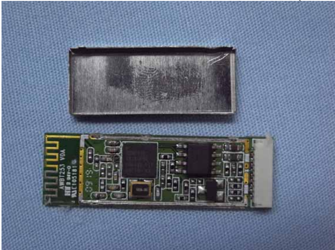
Figure 26 Bluetooth Module (Front View)
