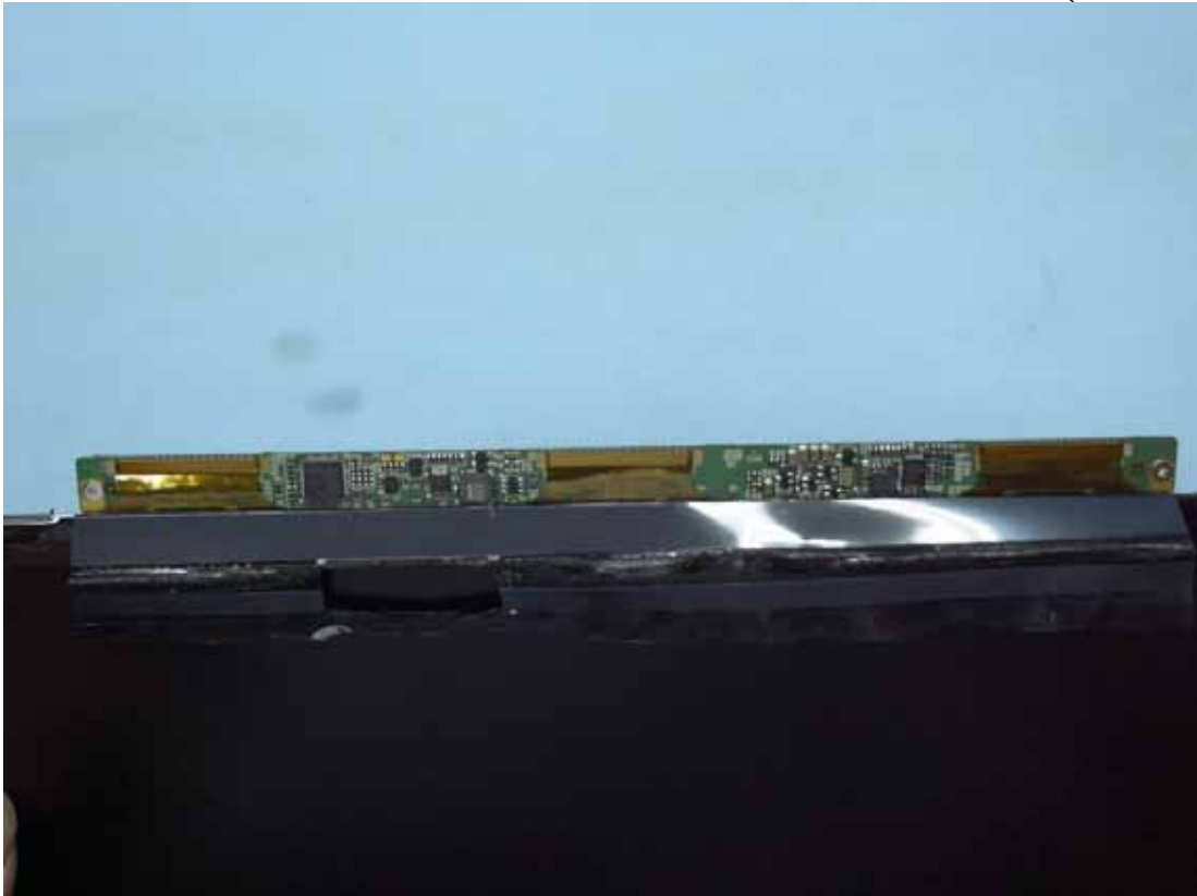
Figure 47 LCD Panel Control Board (Front View)
