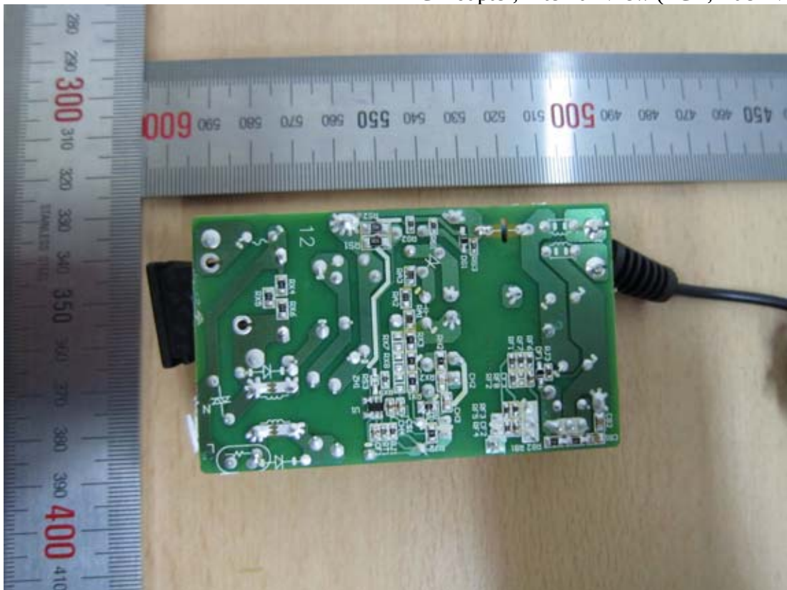
Figure 12 AC Adapter, Internal View (PCB, Back View)
