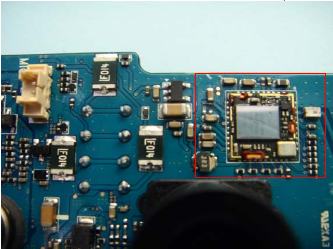
Figure 10 Internal View (WLAN Module)
