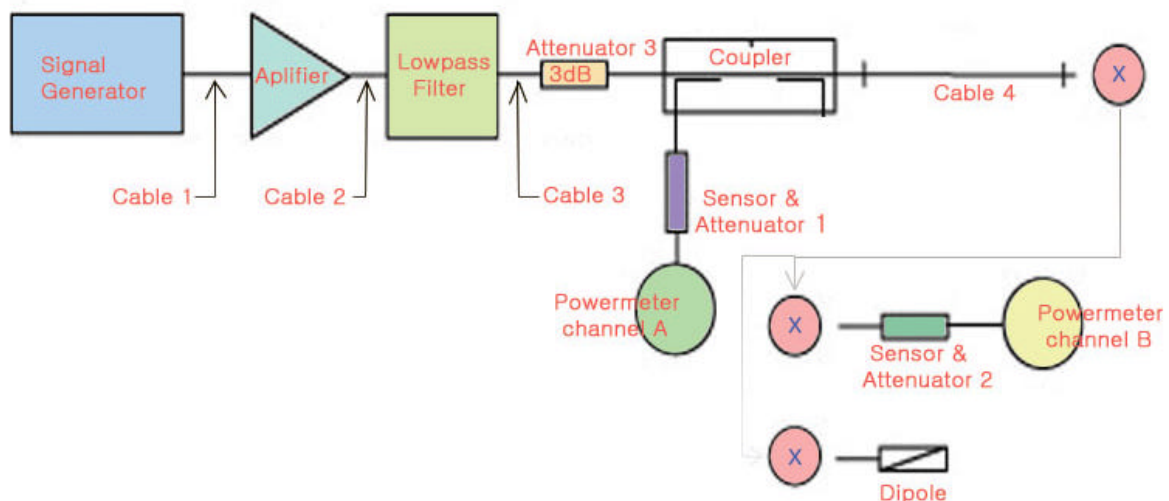
Figure 12.1 Dipole Validation Test Setup
