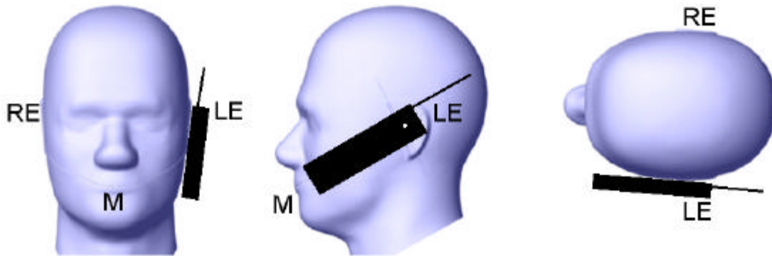
Figure 6.3 "Cheek" or "Touch" Position.
